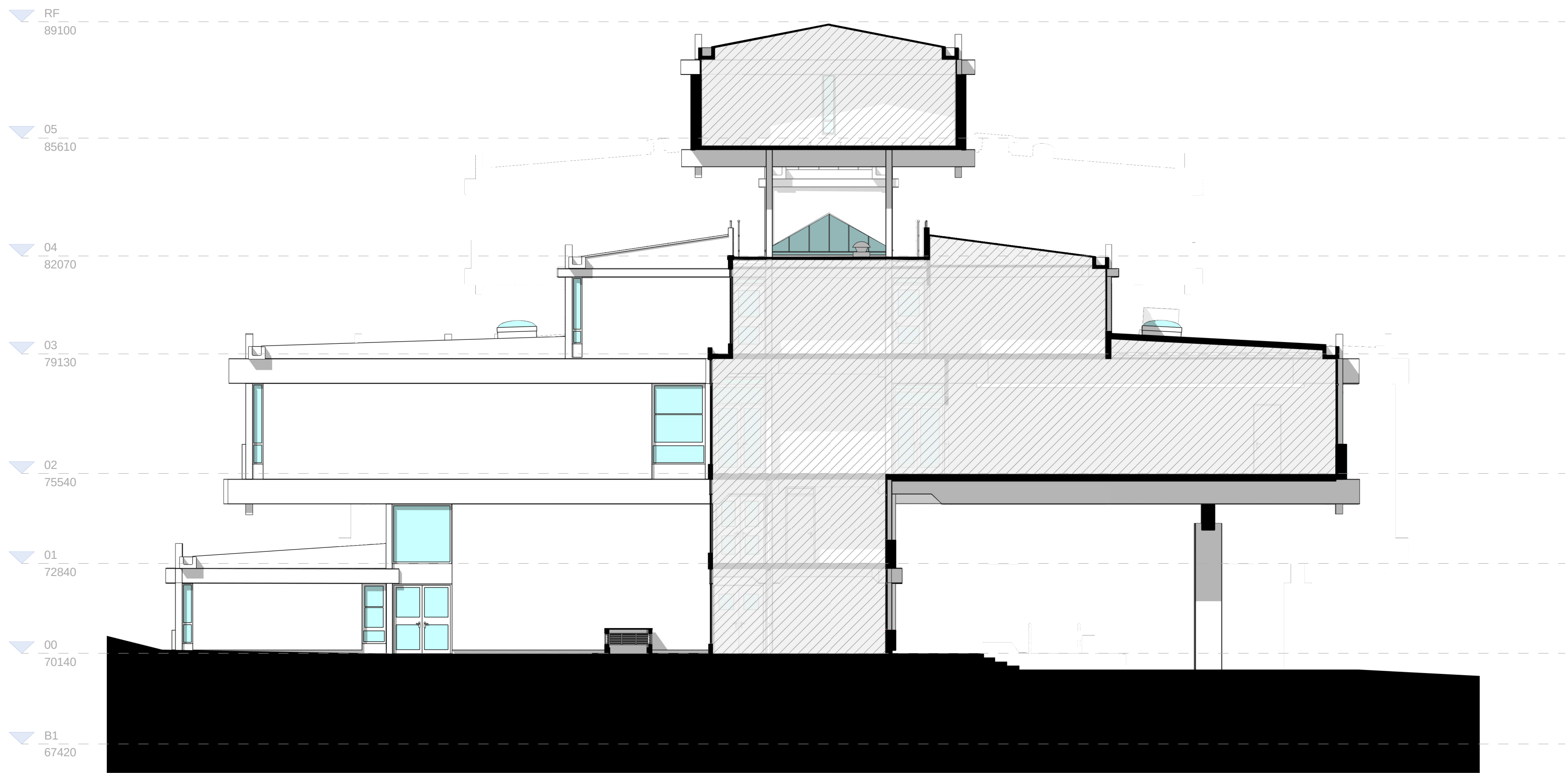
L | 21004-Elevation-Cut-East_LL_Existing 1 : 100
