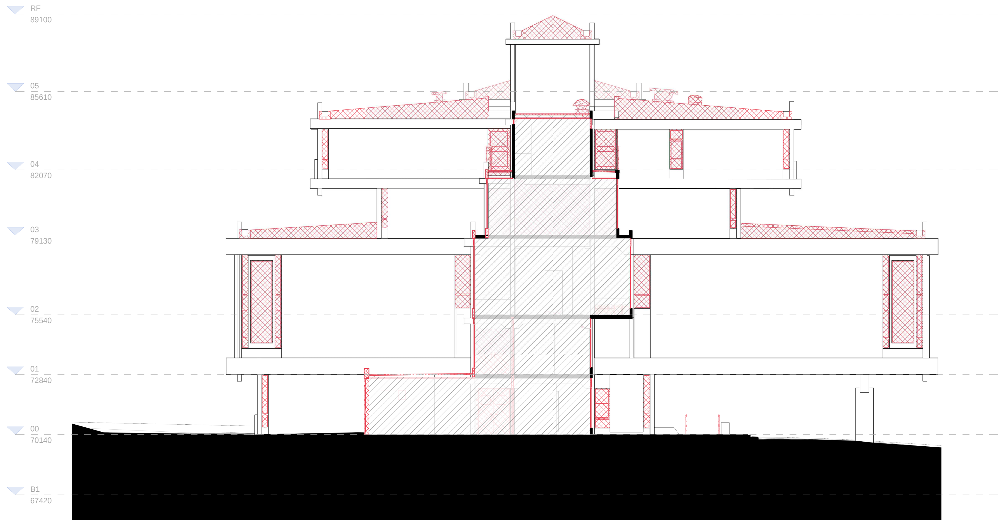
I | 21133-Elevation-Cut_II_Phase3 1:100
