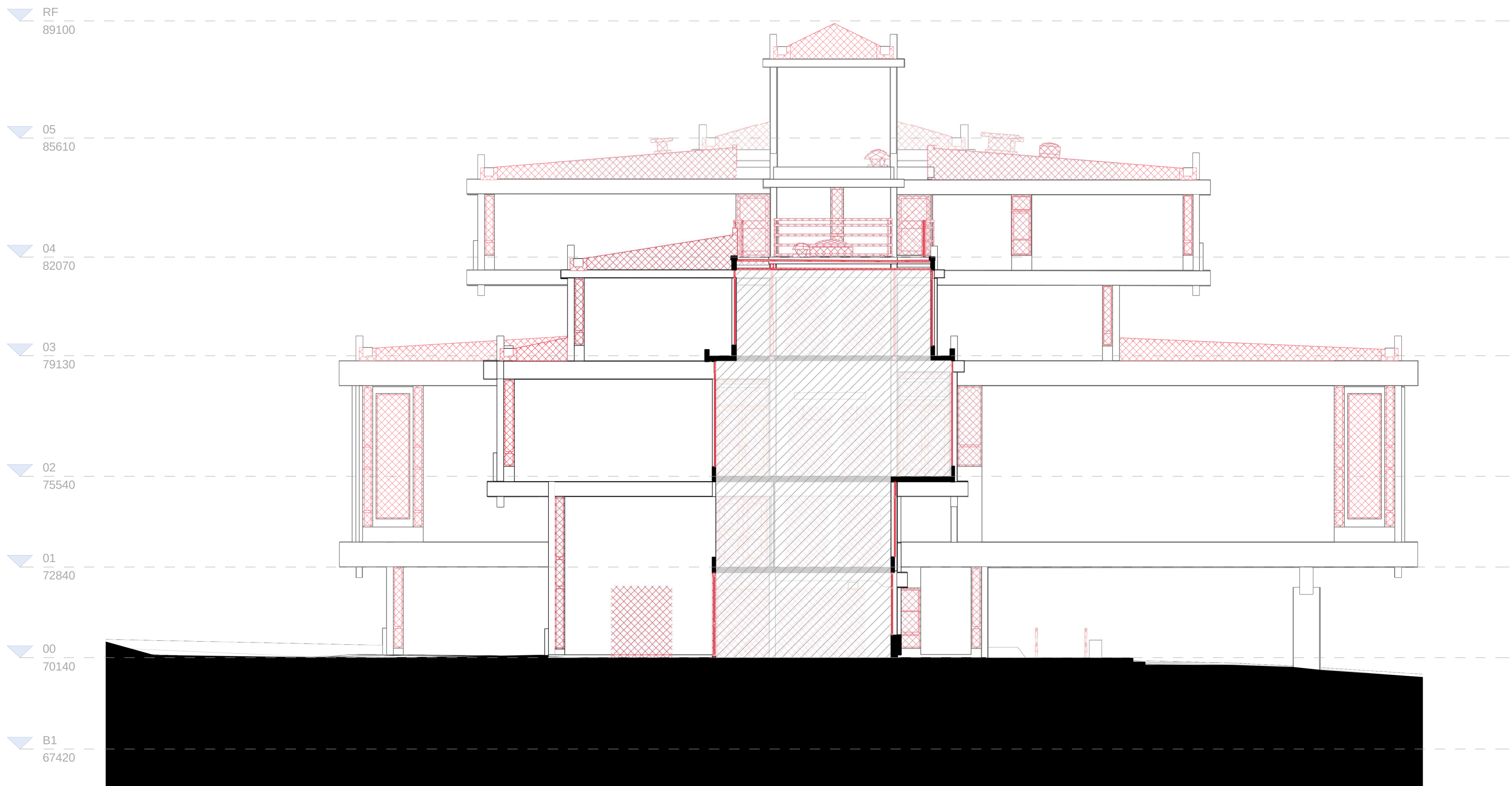
J | 21133-Elevation-Cut-East_JJ_Phase3 1:100
