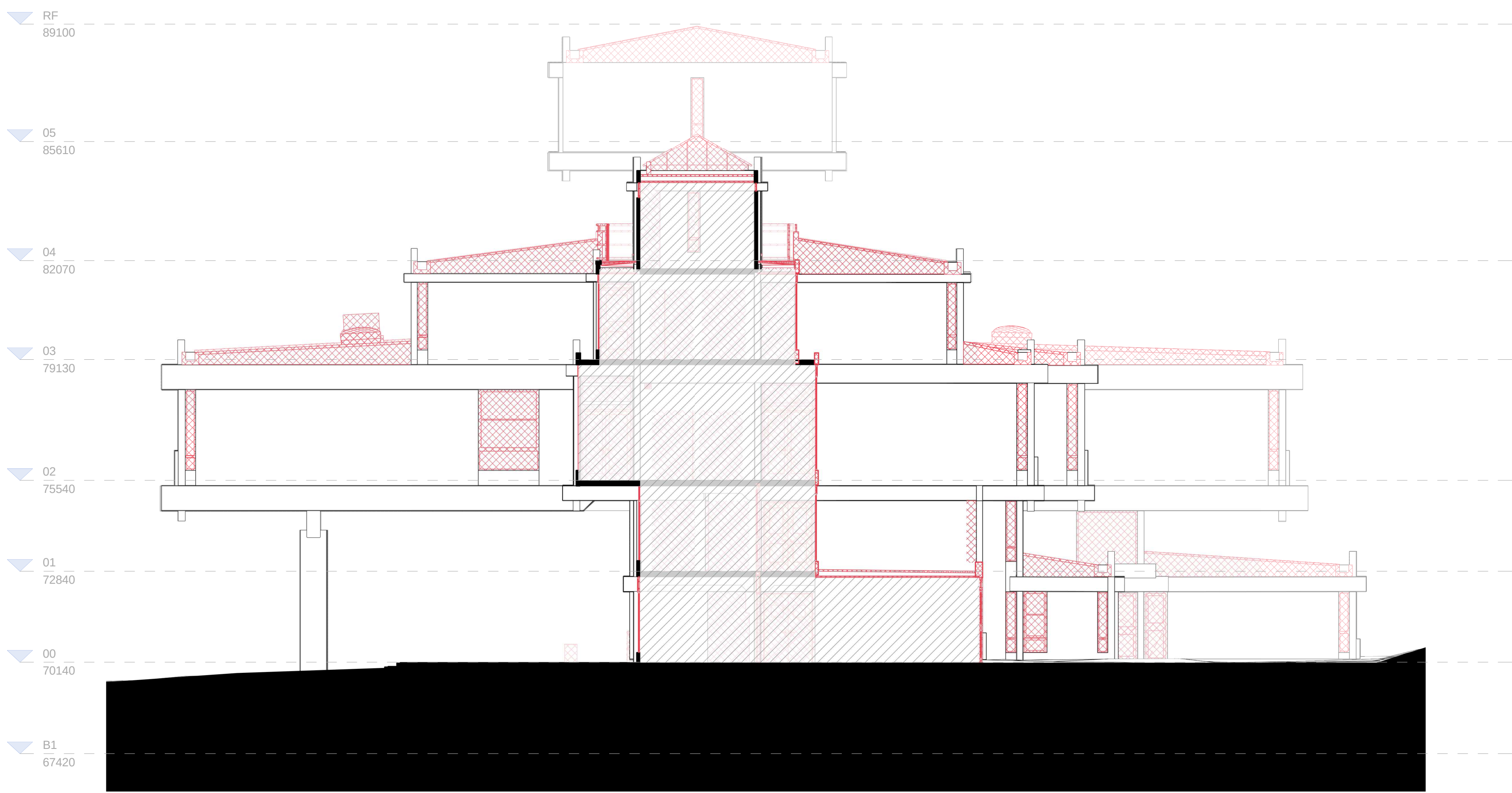
N | 21134-Elevation-Cut-West_NN_Phase3 1 : 100
