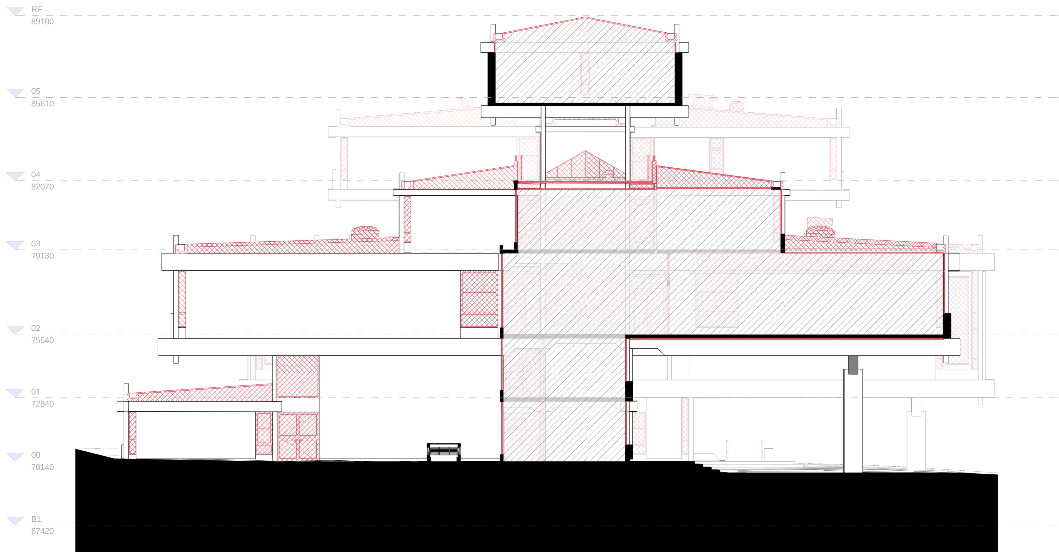
L | 21134-Elevation-Cut-East_LL_Phase3 1 : 100
