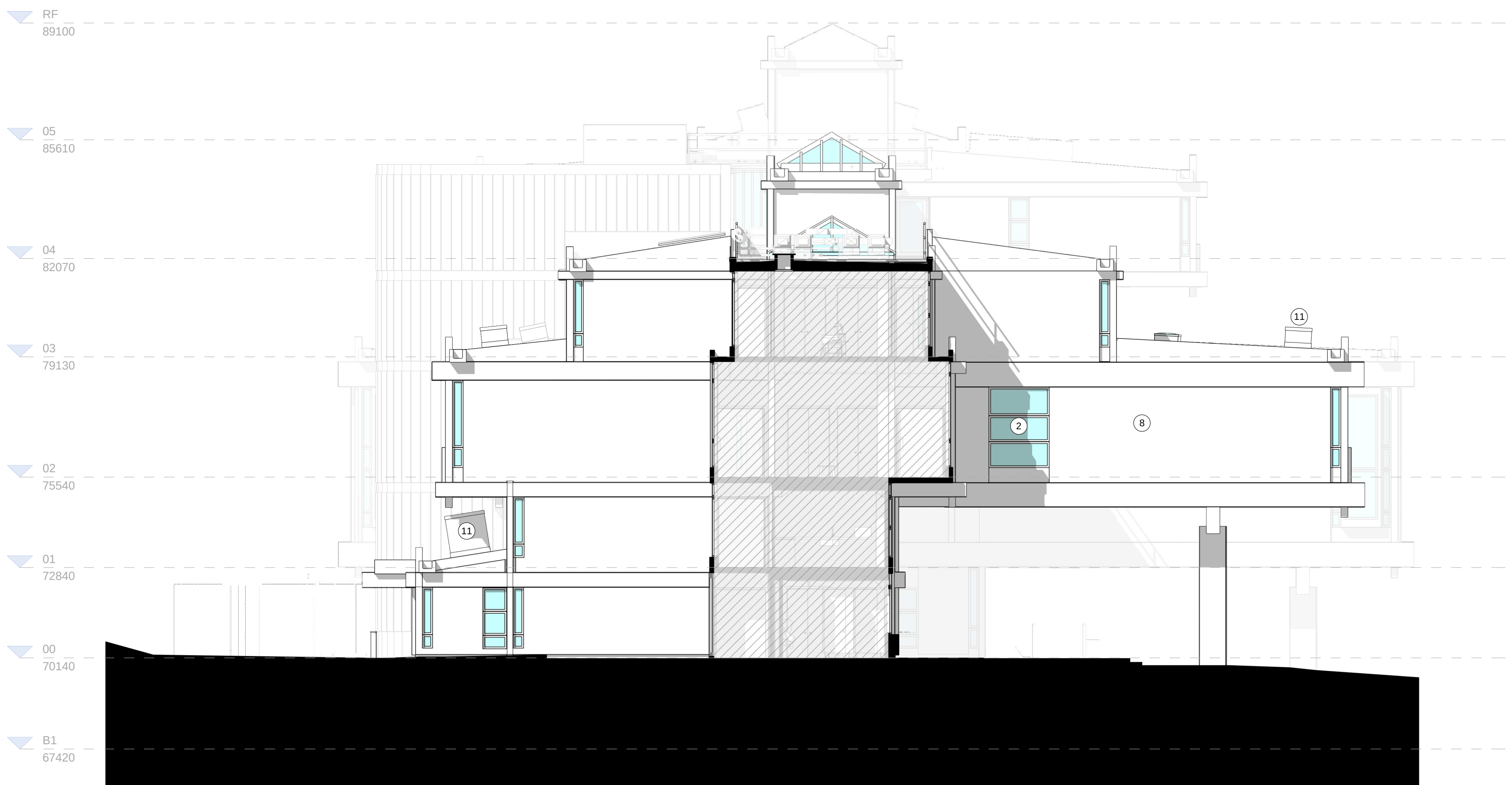
21303-Elevation-Cut-East_KK_Phase3 1:100
