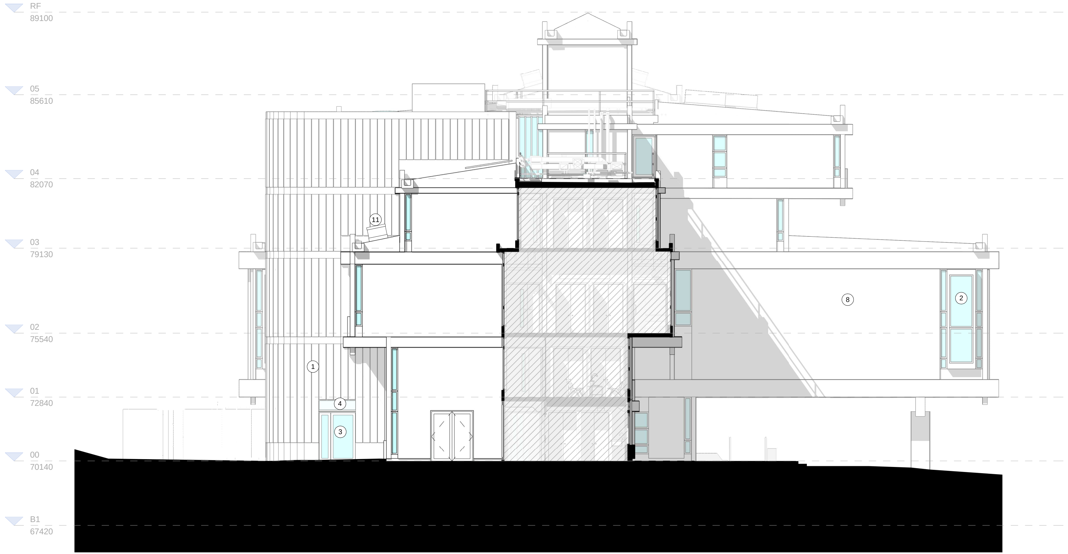
21303-Elevation-Cut-East_JJ_Phase3 1:100
