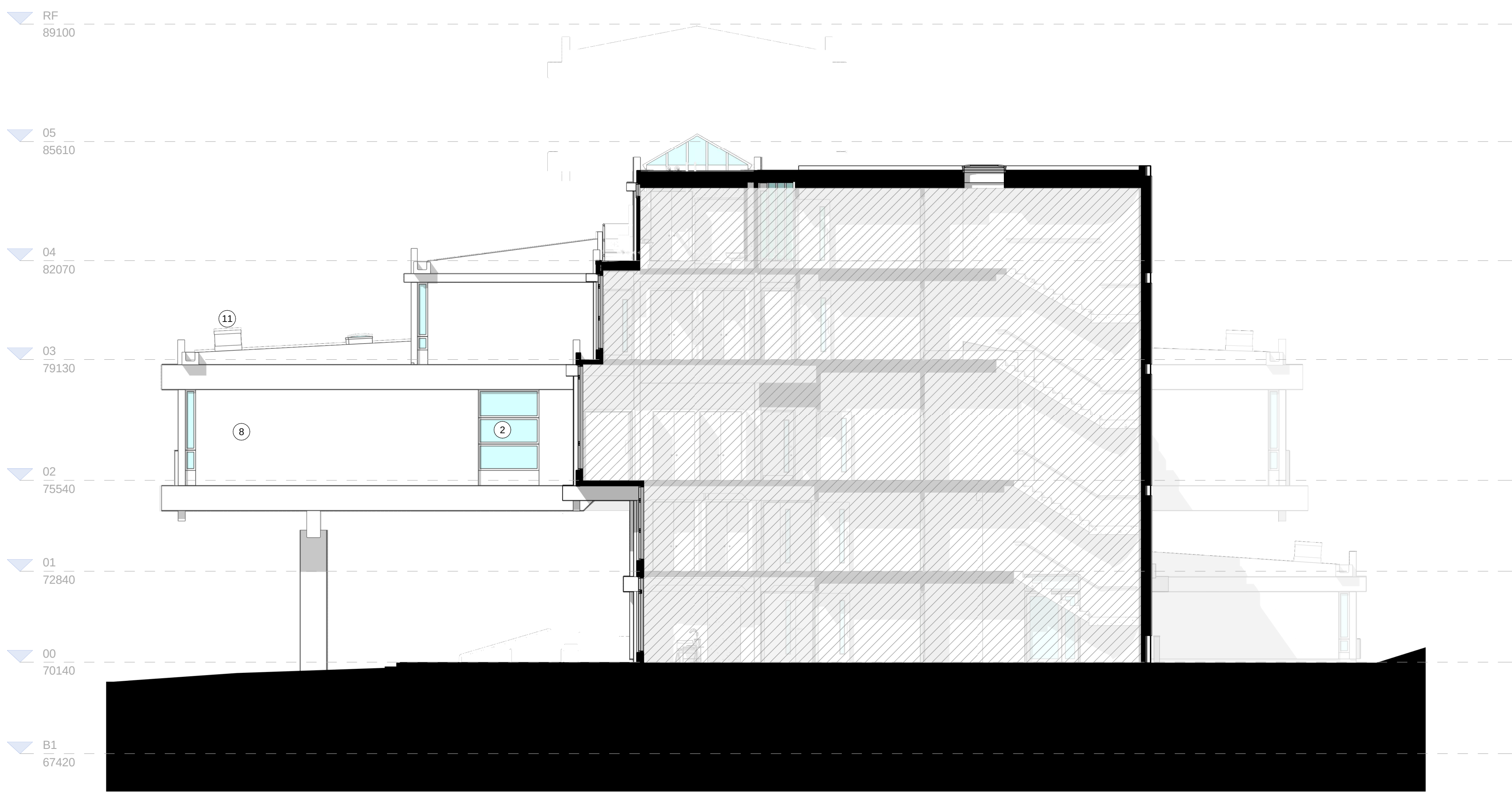
N | 21304-Elevation-Cut-West_NN_Phase3 1 : 100
