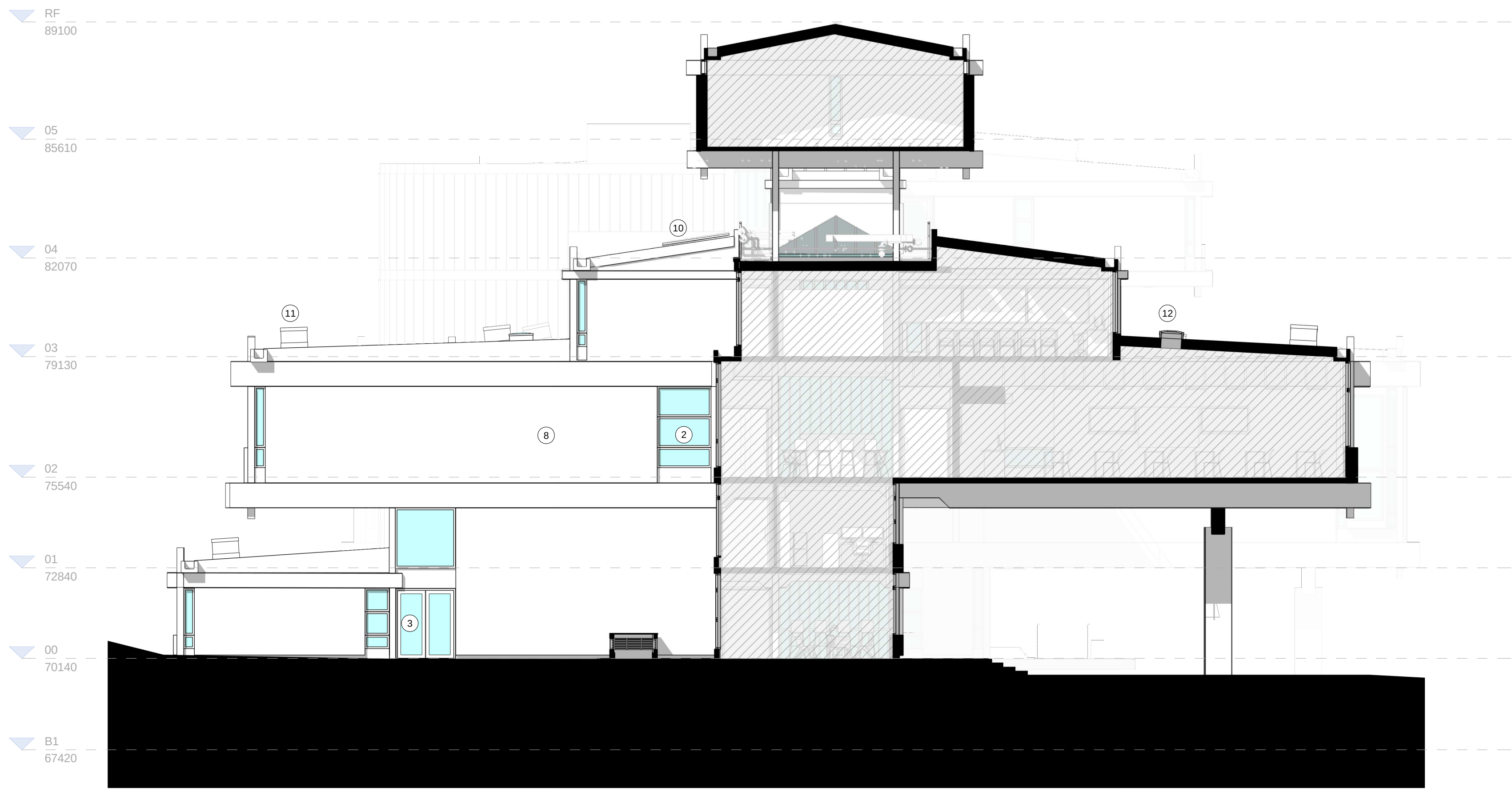
L | 21304-Elevation-Cut-East_LL_Phase3 1 : 100
