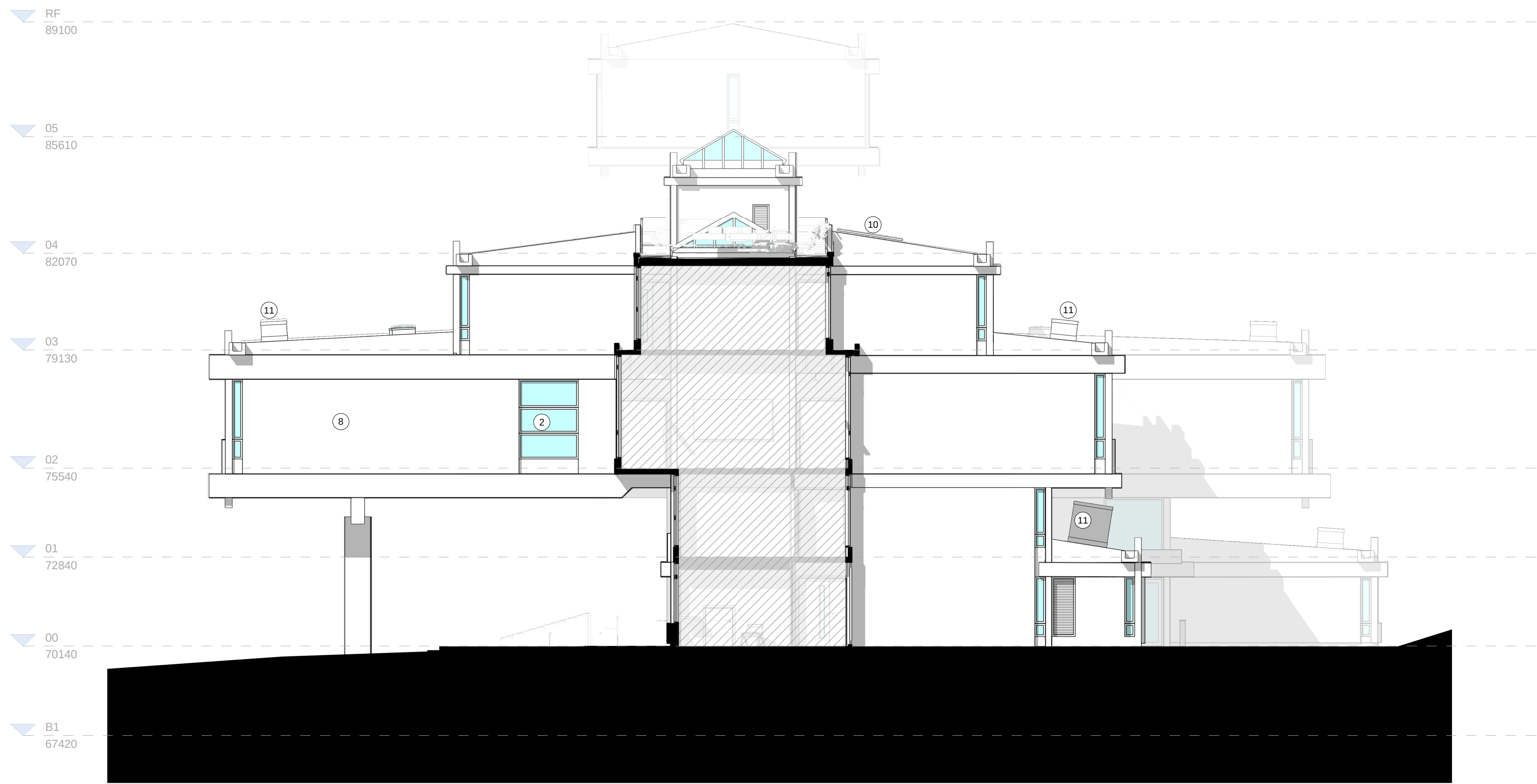
O | 21305-Elevation-Cut-West_OO_Phase3 1:100
