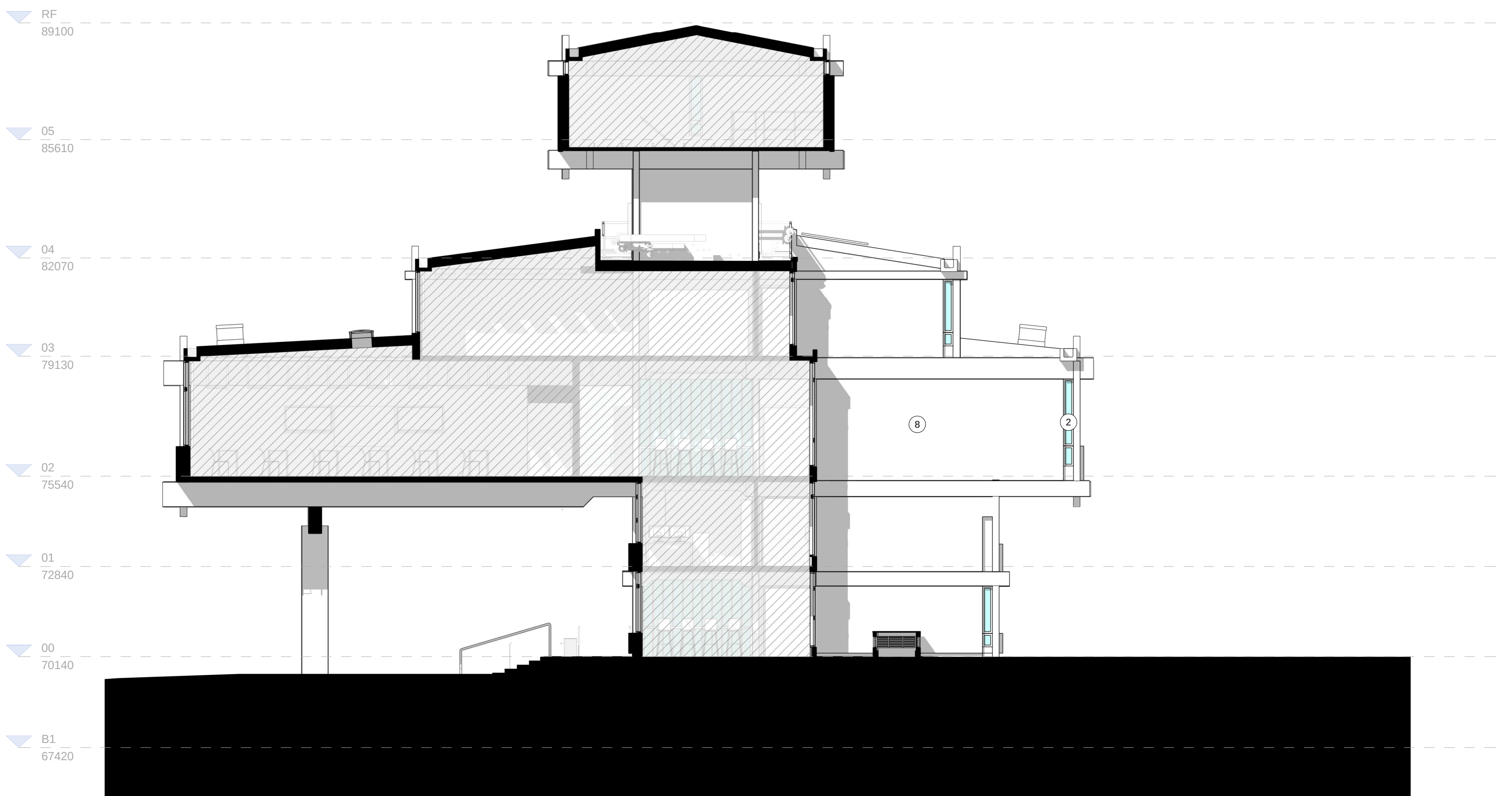
Q | 21305-Elevation-Cut-West_QQ_Phase3 1:100
