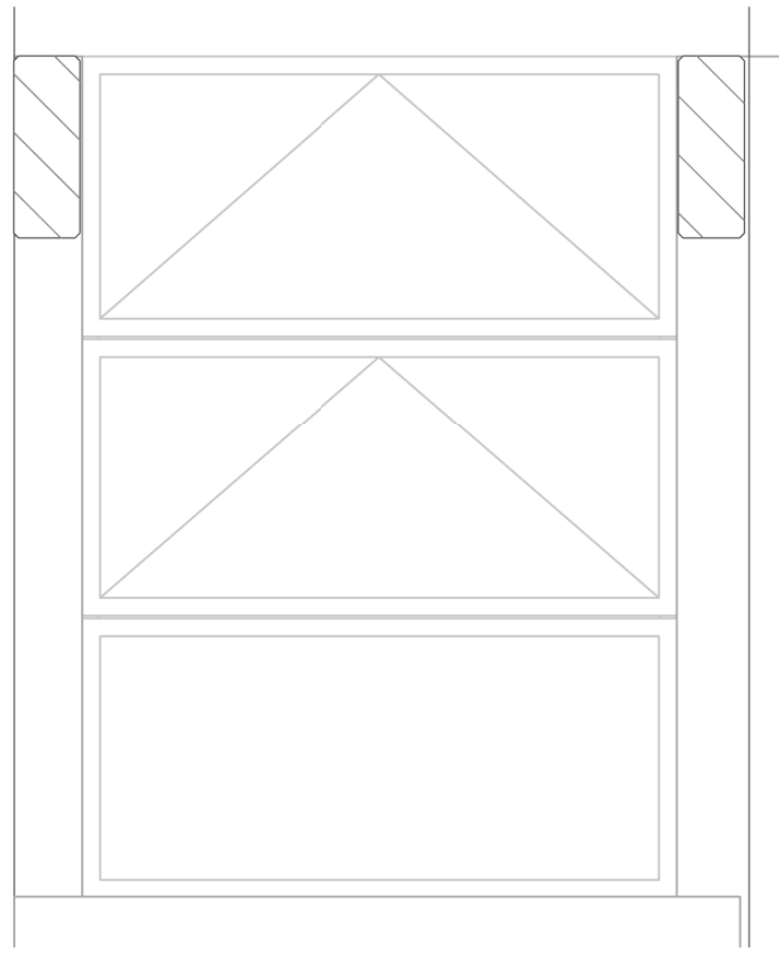
Proposed Window Type-1x3 (South) 1 : 25
