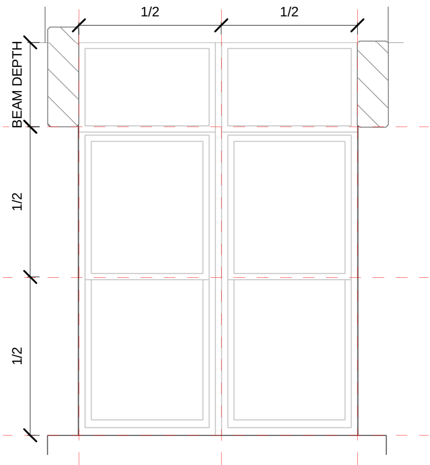
Existing Window Type-2x3 (South) 1 : 25
