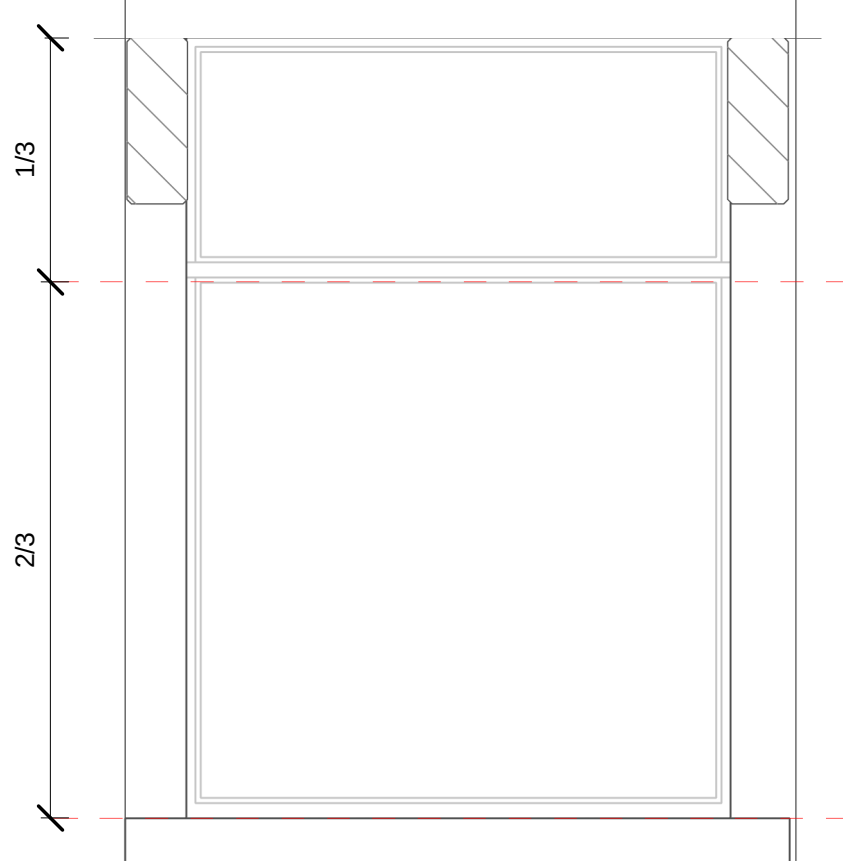
Existing Window Type-1x2 (South) 1 : 25
