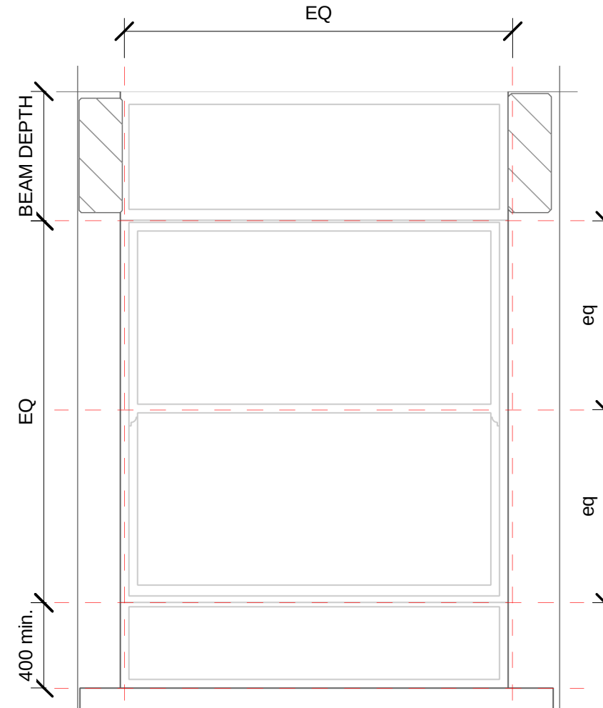
Existing Window Type-1x4 (South) 1 : 25
