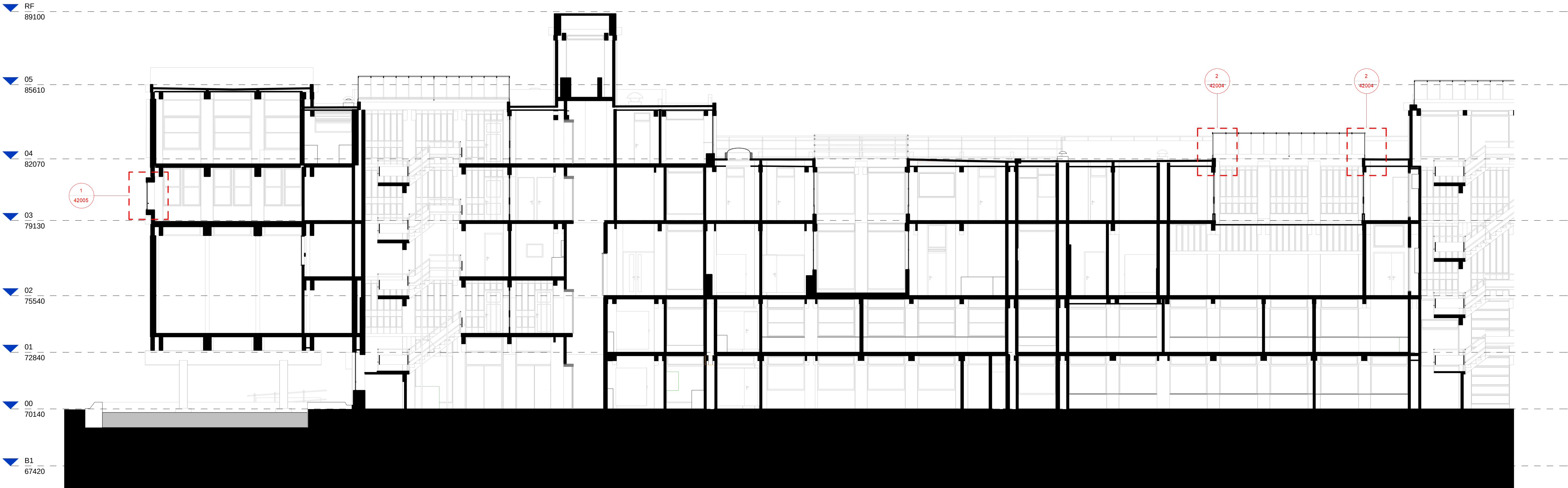
3 30000-Existing Section AA_West 1:100
