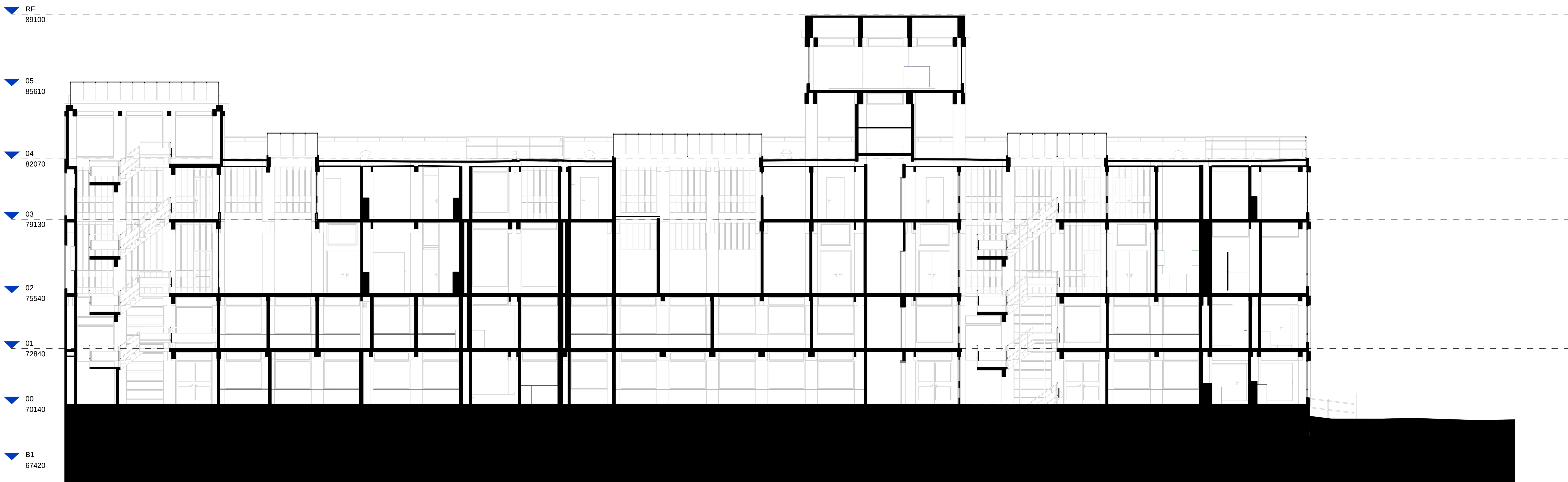
2 30000-Existing Section AA_East 1:100
