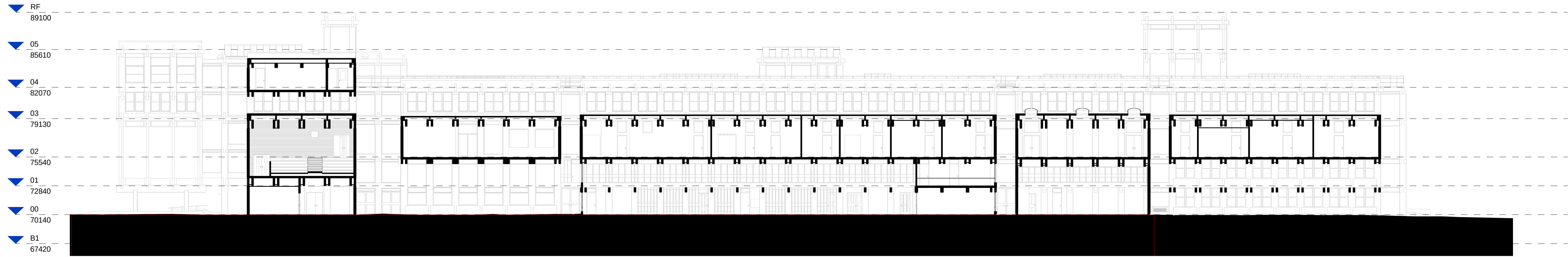
FF | 30002-Existing Section FF_ALL 1 : 200
