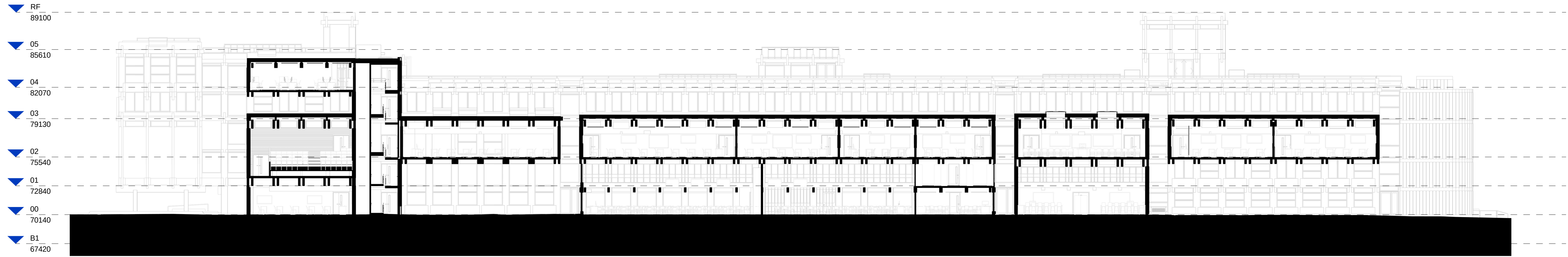
FF | 30302-Section FF_ALL 1 : 200
