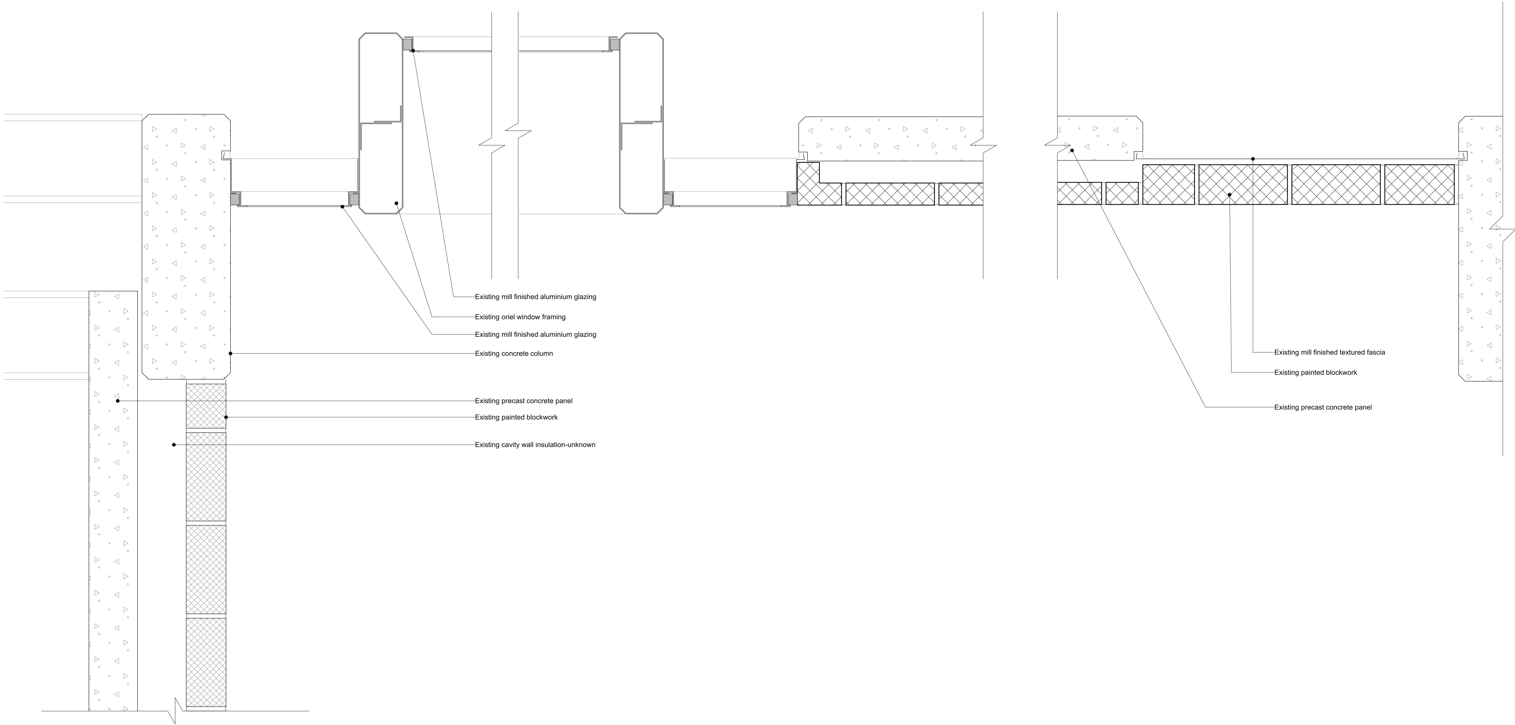
1 Oriel Window Plan Detail - Existing Scale: 1:5
