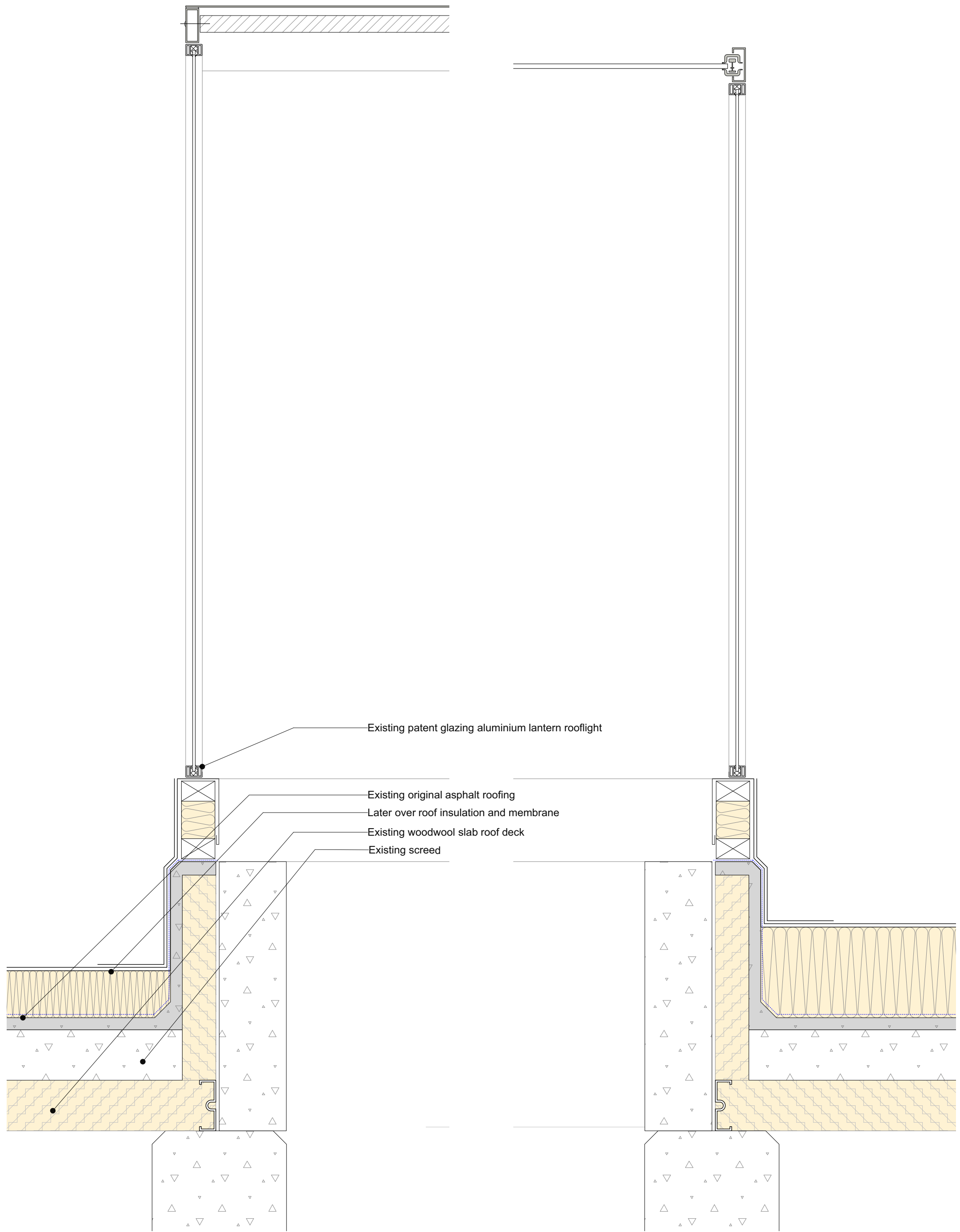
2 Lantern Ridge / Verge Section Detail - Existing Scale: 1:5
