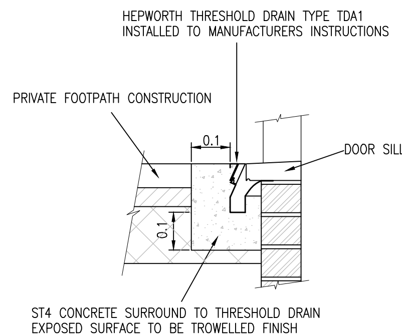
THRESHOLD DRAIN DETAIL (TD) OR SIMILAR APPROVED
