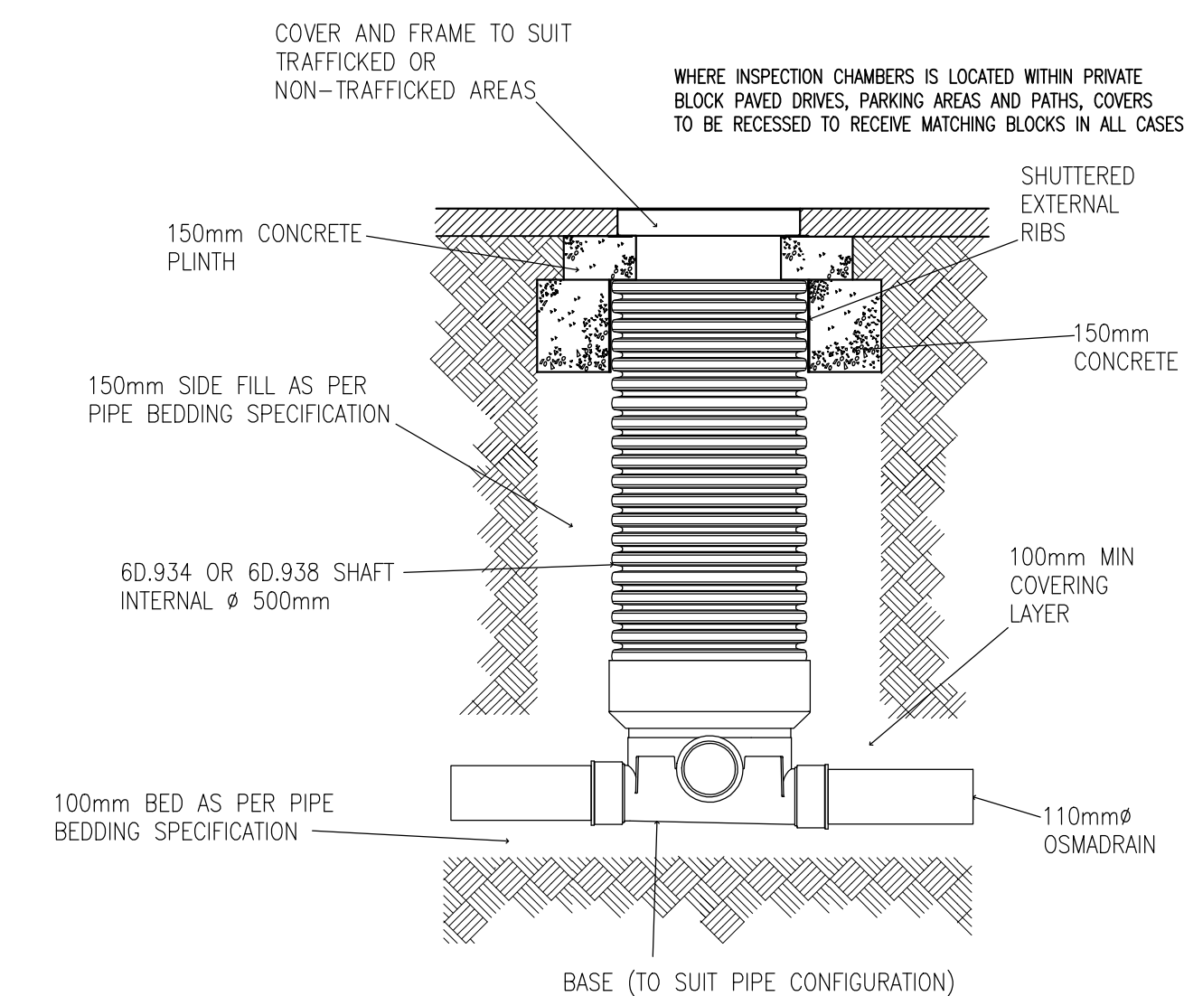
MAXIMUM DEPTH 3.0m TO BE INSTALLED TO MANUFACTURERS INSTALLATION GUIDE
