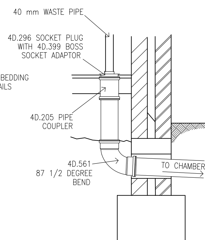
STUB STACK CONNECTION
