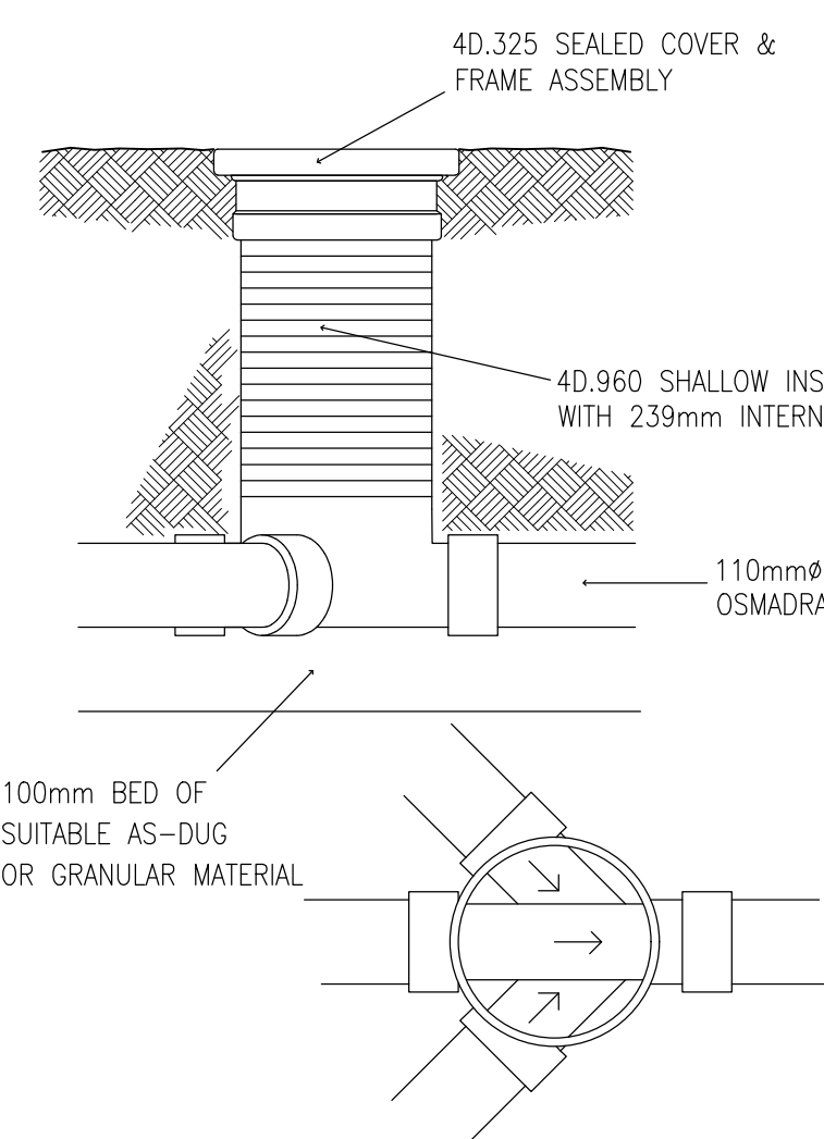
MAXIMUM DEPTH 0.6m TO BE INSTALLED TO MANUFACTURERS INSTALLATION GUIDE
