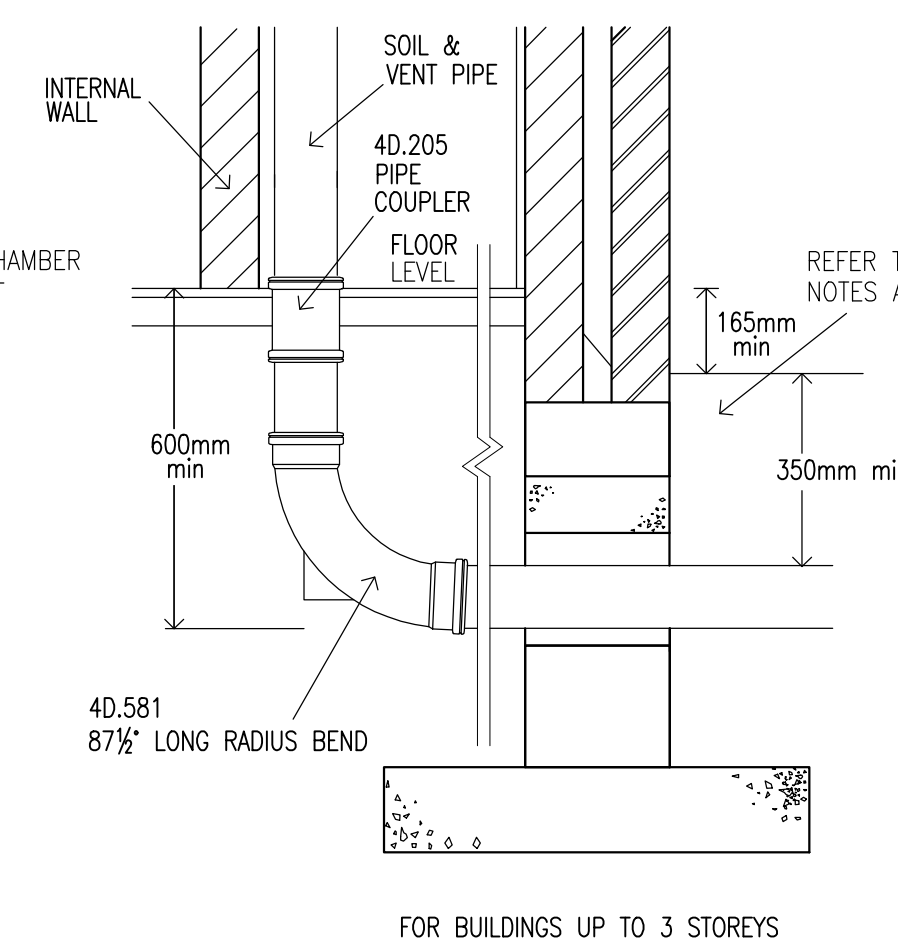
FOR BUILDINGS UP TO 3 STOREYS
