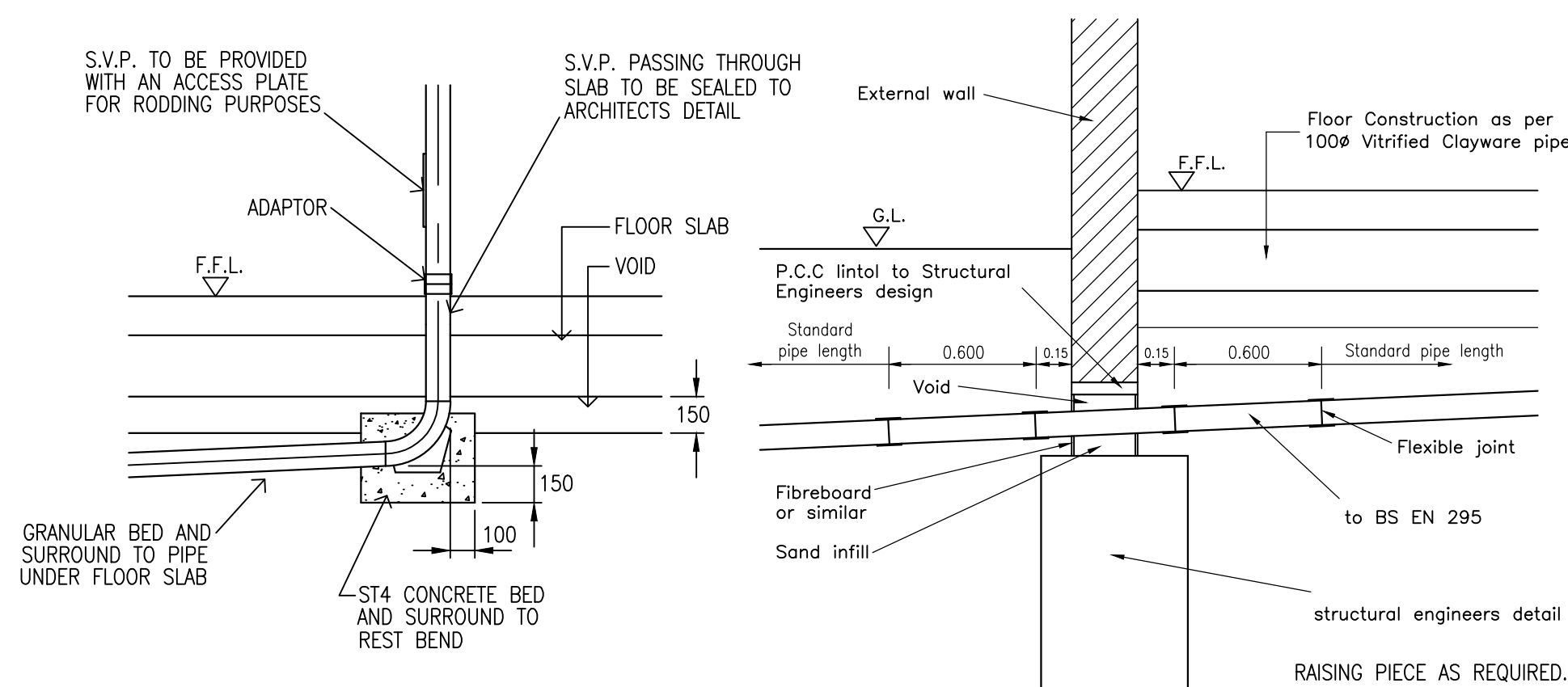
SVP PASSING THROUGH FLOOR SLAB
