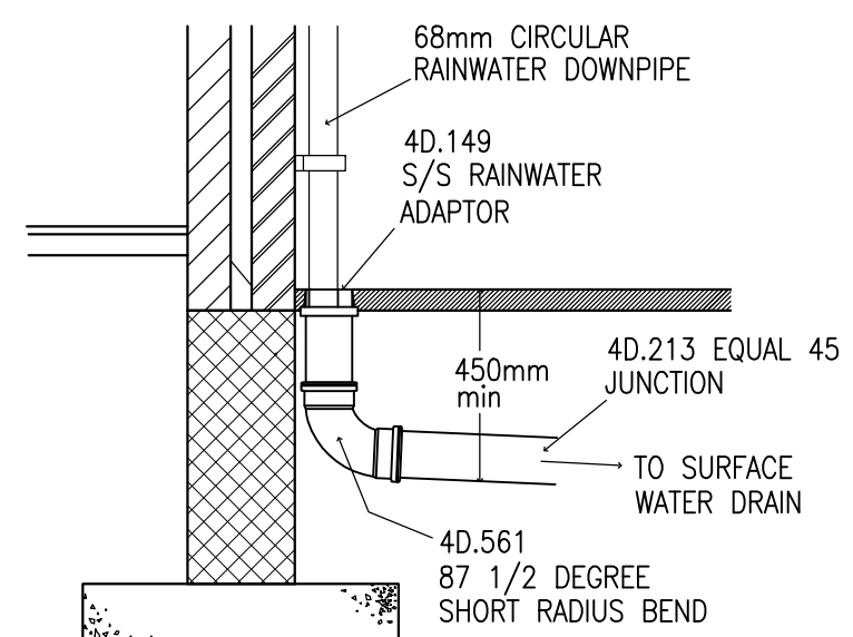
EXTERNAL RWP OUTLET
