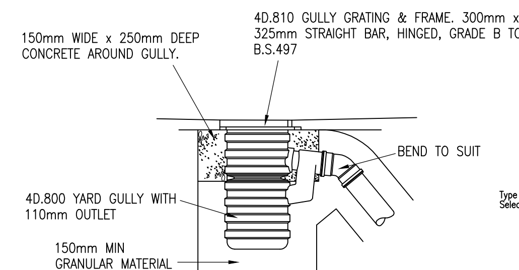
THRESHOLD DRAIN DETAIL (TD) OR SIMILAR APPROVED
