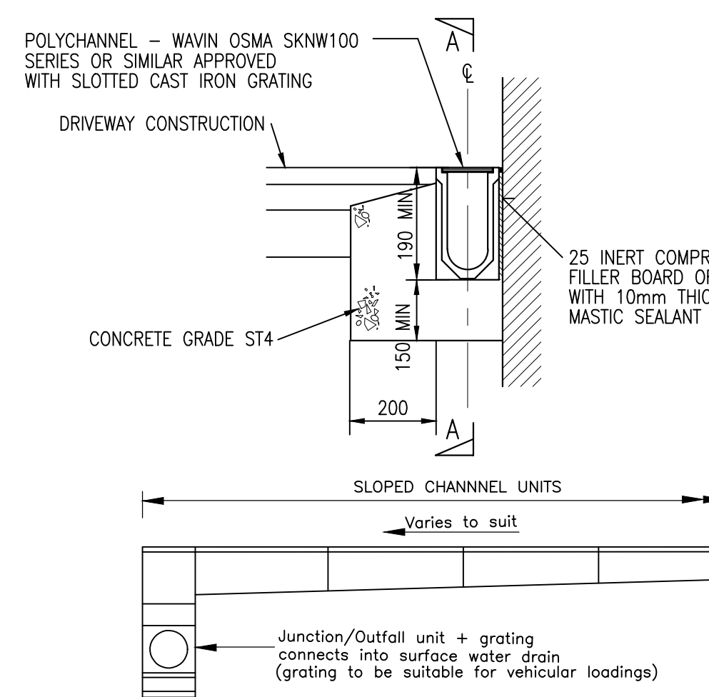
LINEAR DRAIN DETAIL (LD) ADJACENT TO FRONT OF GARAGES
