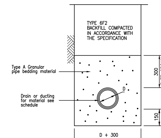
BEDDING CLASS S
