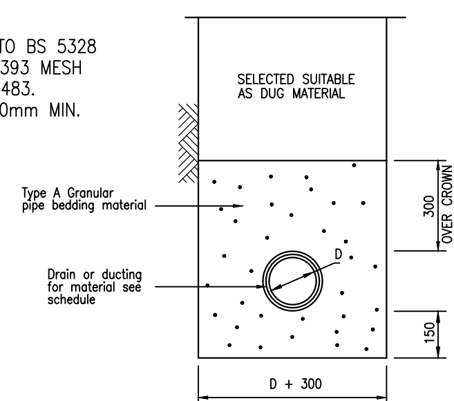
BEDDING CLASS S1 FOR DRAINAGE UNDER SOFT AREAS
