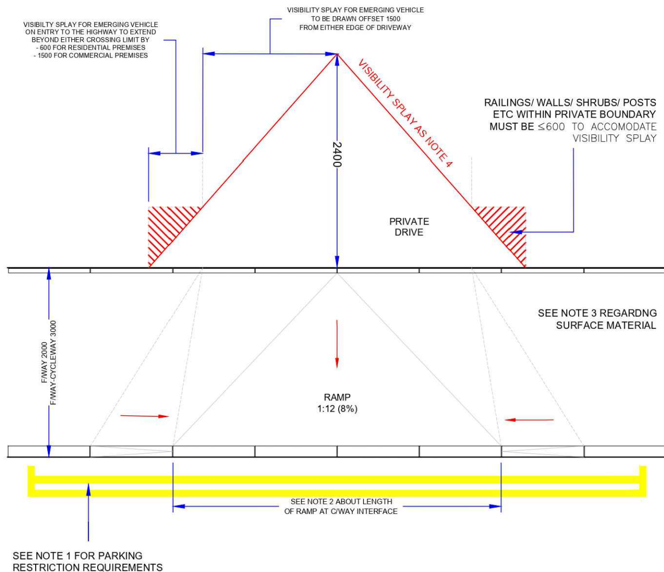
VEHICULAR CROSSING TYPE 1
