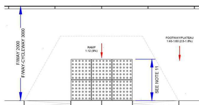
INSET TACTILE PAVING PEDESTRIAN CROSSING POINT AWAY FROM JUNCTIONS
