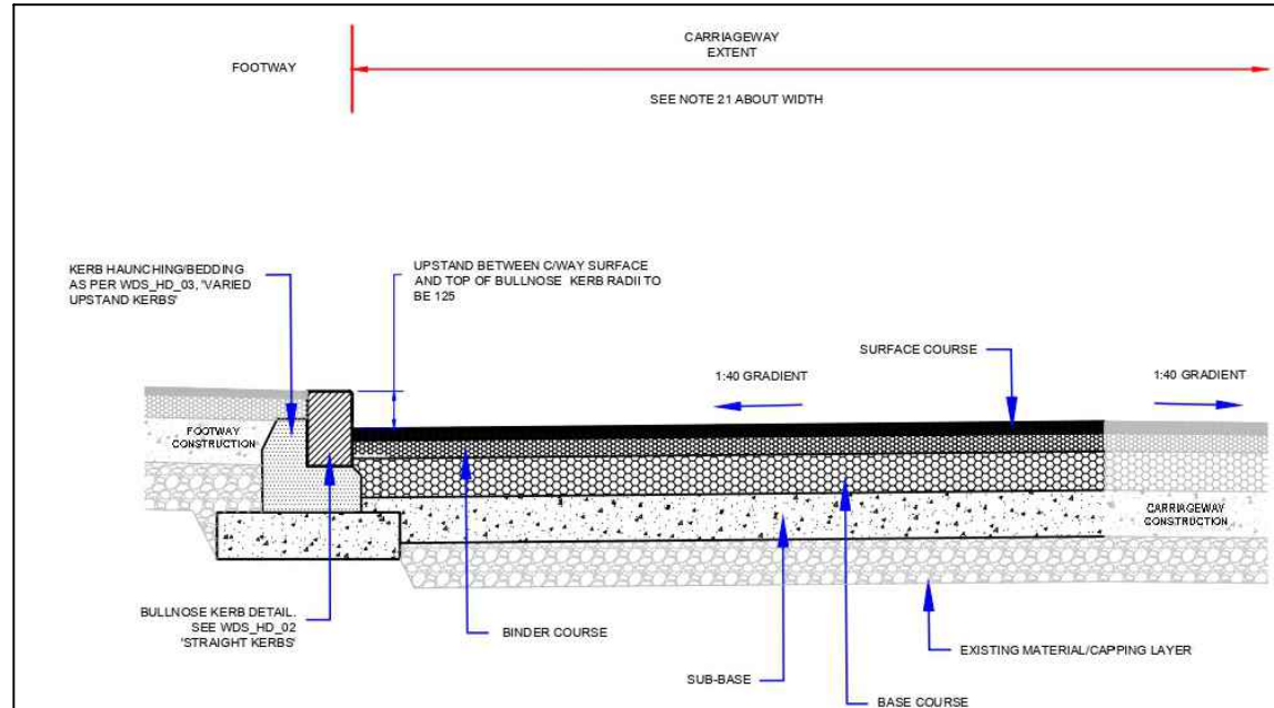
TARMACADAM CARRIAGEWAY SEE TABLE FOR CONSTRUCTION DETAILS
