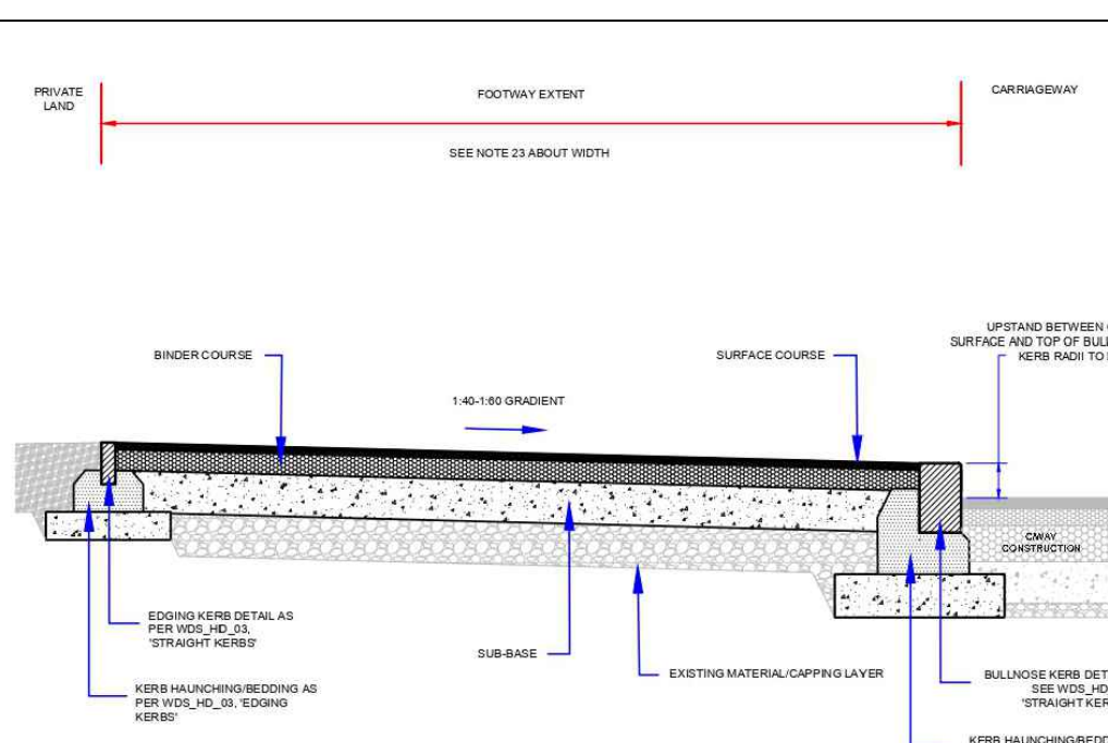
TARMACADAM FOOTWAY/CYCLEWAY SEE TABLE FOR CONSTRUCTION DETAILS
