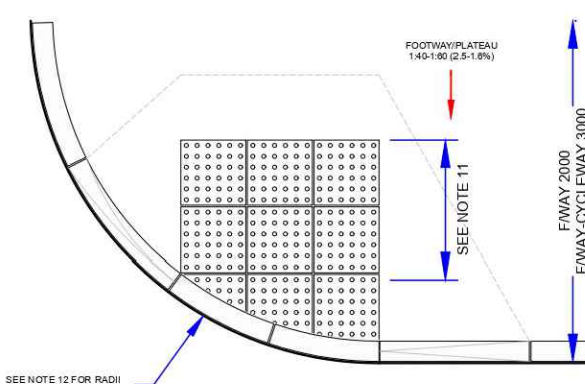
TACTILE PAVING PEDESTRIAN CROSSING AT JUNCTION
