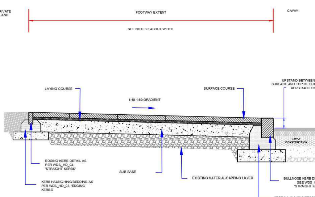
MODULAR PAVING FOOTWAY SEE TABLE FOR CONSTRUCTION DETAILS
