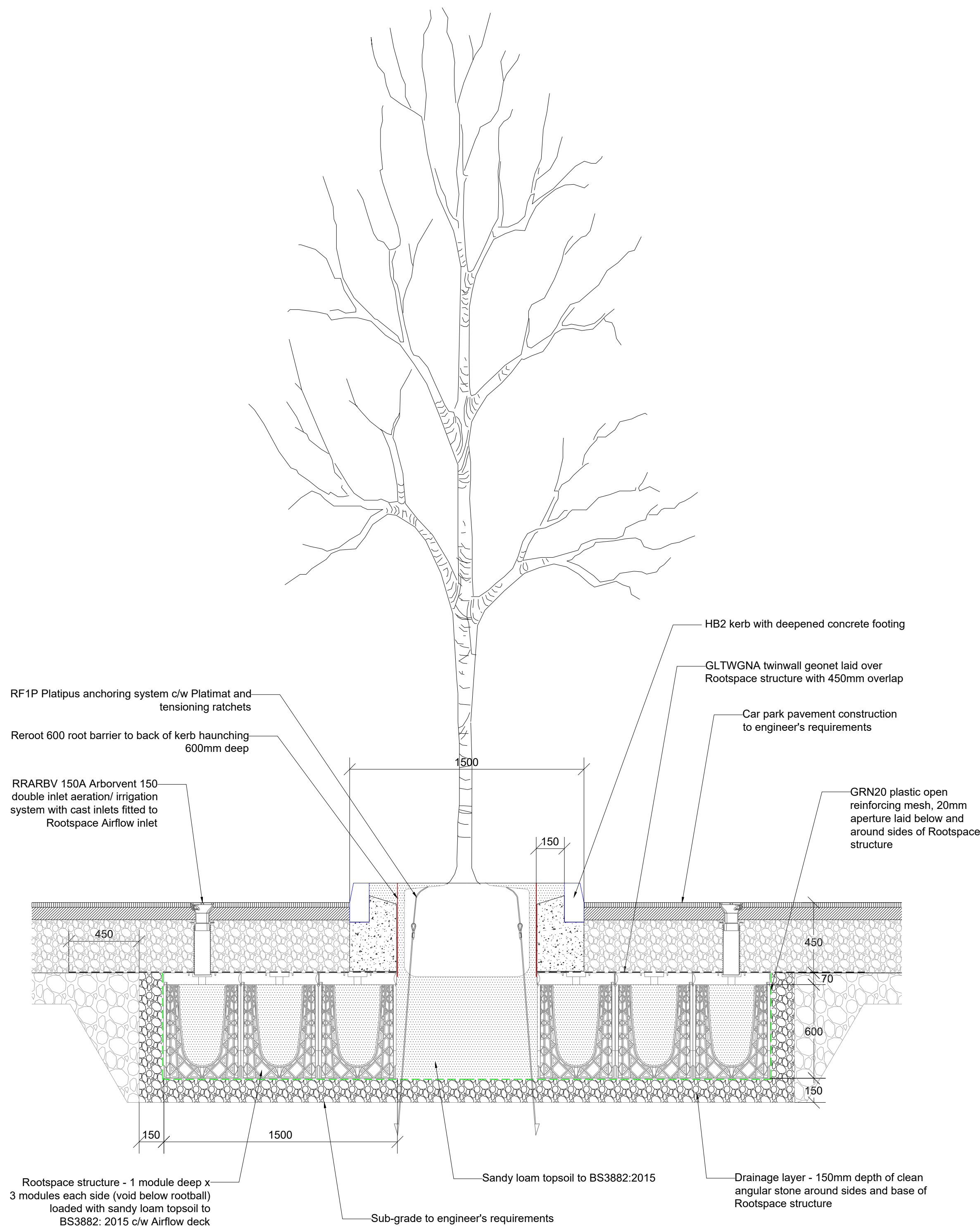
Tree Pit in Restricted Area of Soft landscape with Crate Detail
