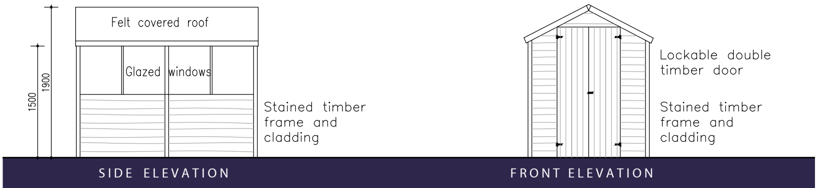
CAR & CYCLE PARKING STANDARD DOCUMENT. Design in accordance with section 4.7- CYCLE PARKING DESIGN
