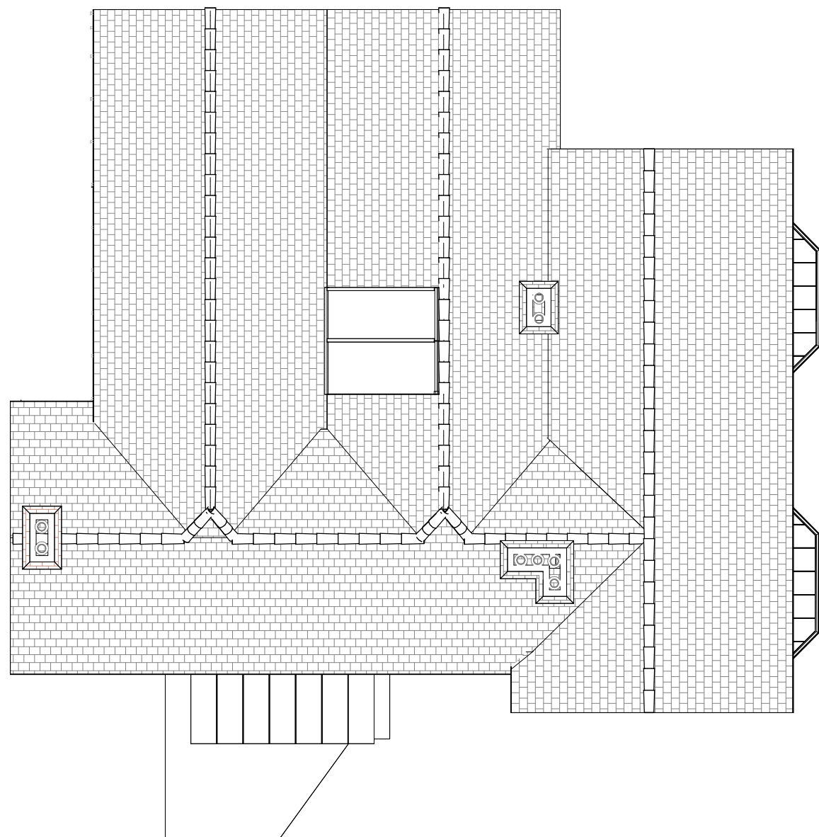
Roof Plan
