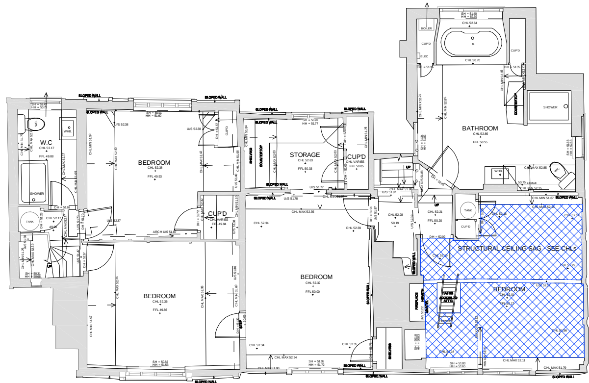
2 PROPOSED FIRST FLOOR REFLECTED CEILING PLAN
