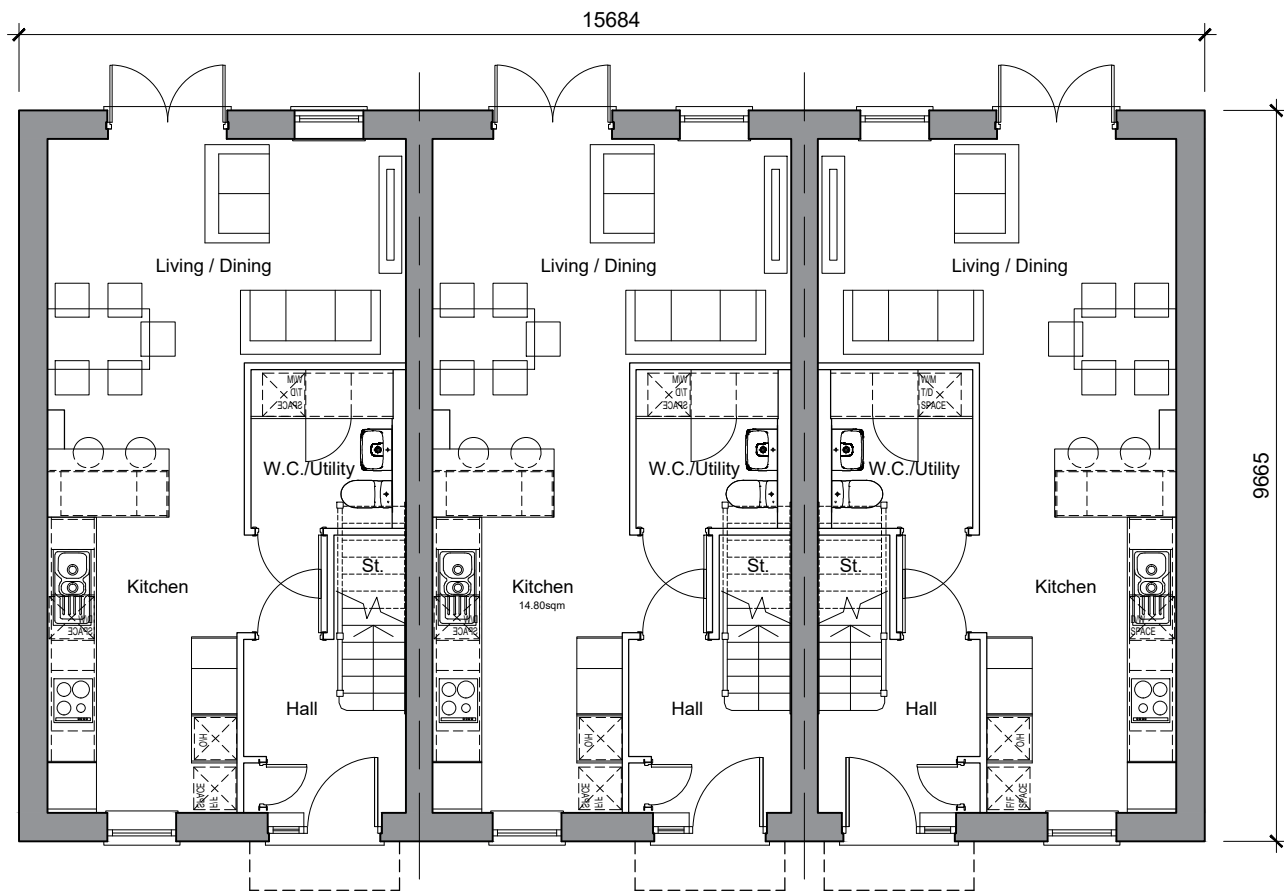
PH3D - 3 Bedroom House NA 113.82sqm
