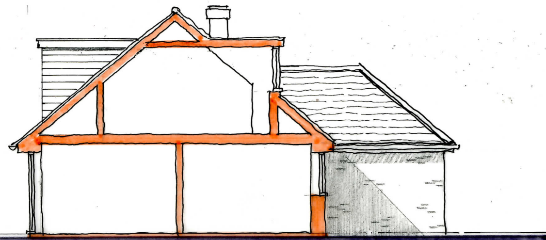
SECTION
