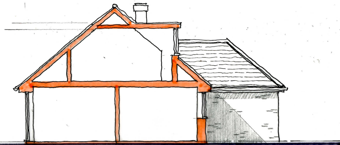
SECTION
