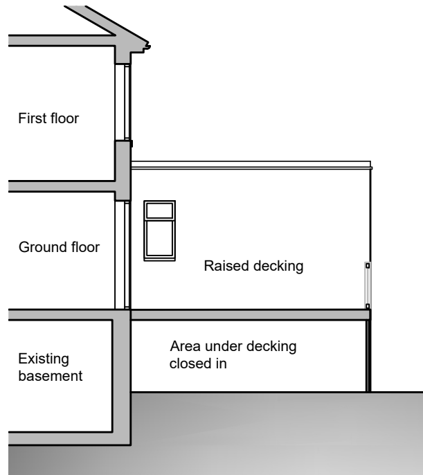
Existing West Sectional Elevation
