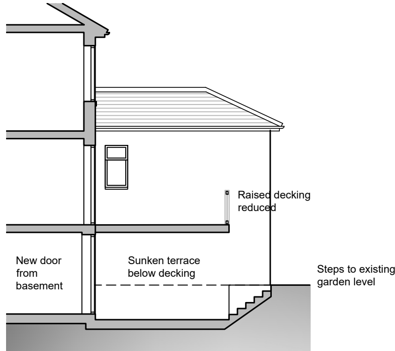
West Sectional Elevation
