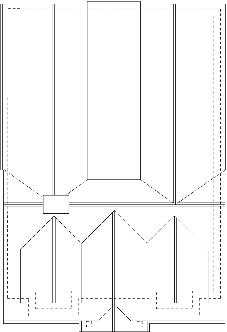
ROOF PLAN
