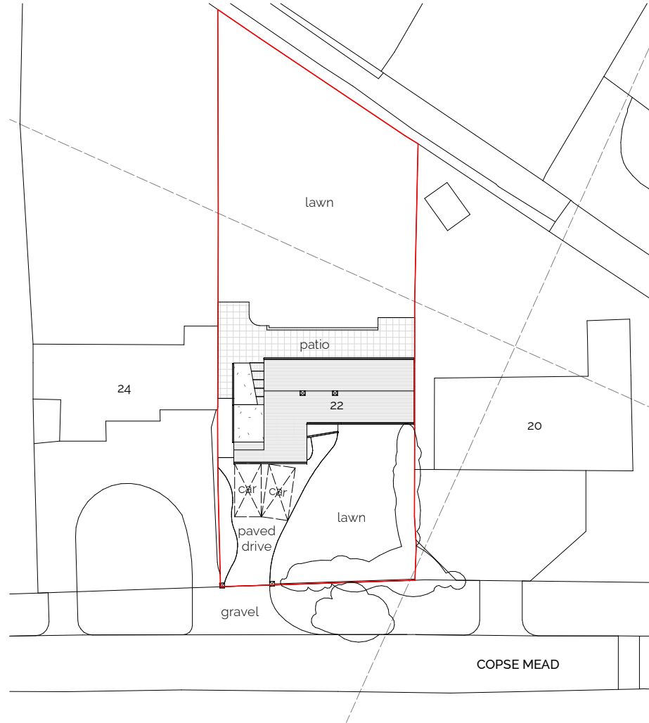
EXISTING SITE BLOCK PLAN Scale 1 : 500
