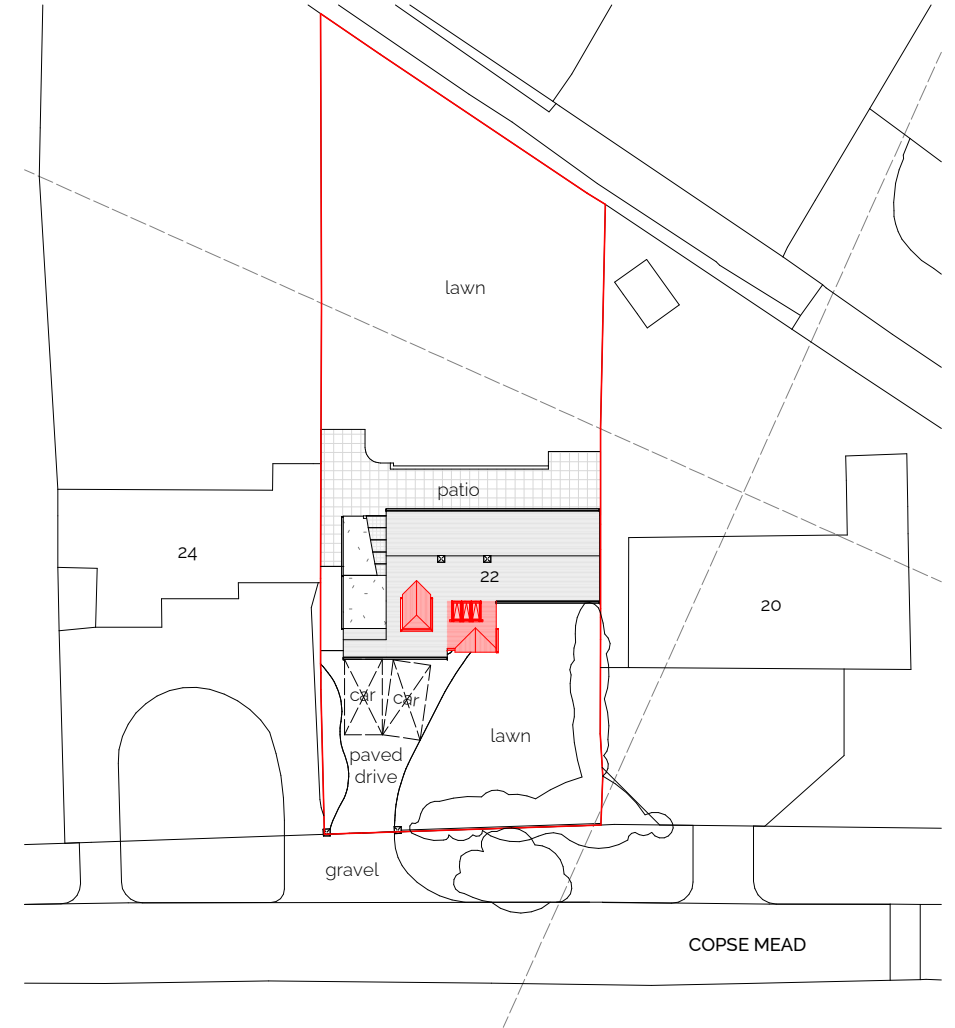
PROPOSED SITE BLOCK PLAN Scale 1 : 500
