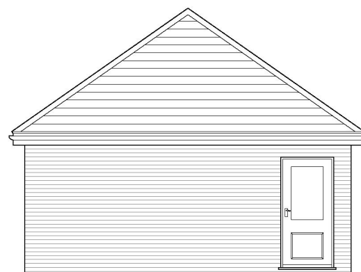
REAR ELEVATION
