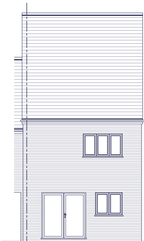
REAR ELEVATION
