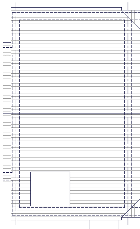
ROOF PLAN
