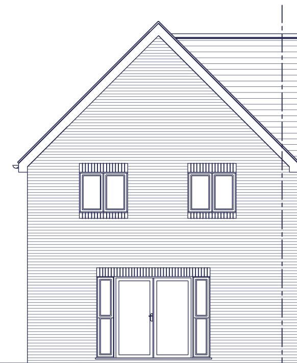
REAR ELEVATION
