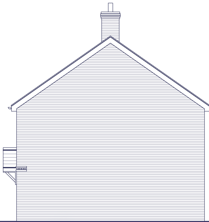
SIDE ELEVATION
