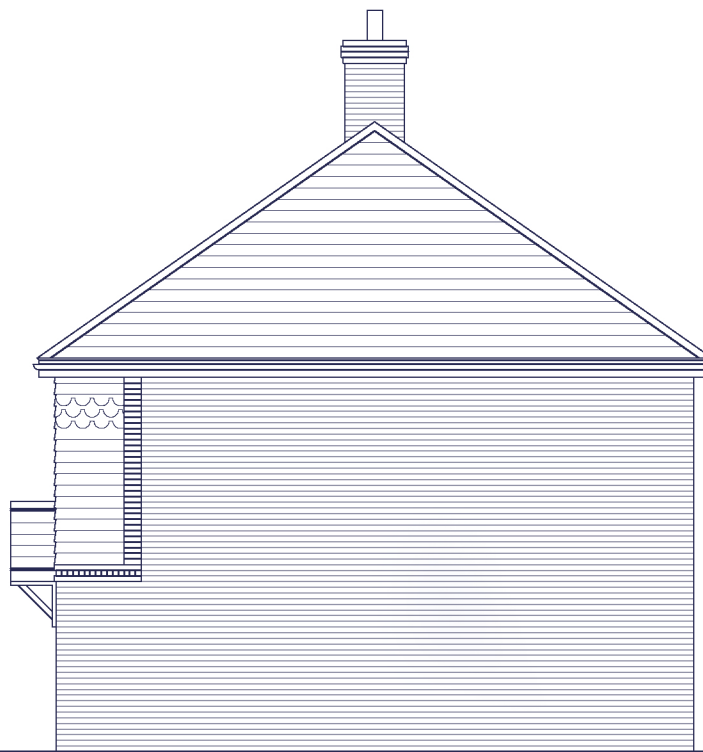
SIDE ELEVATION
