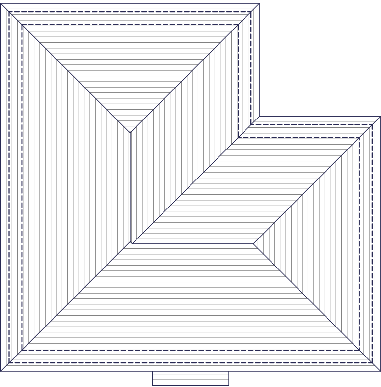
ROOF PLAN
