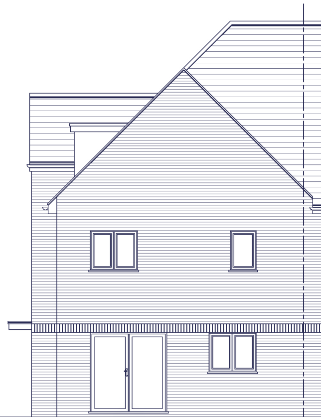
SIDE ELEVATION
