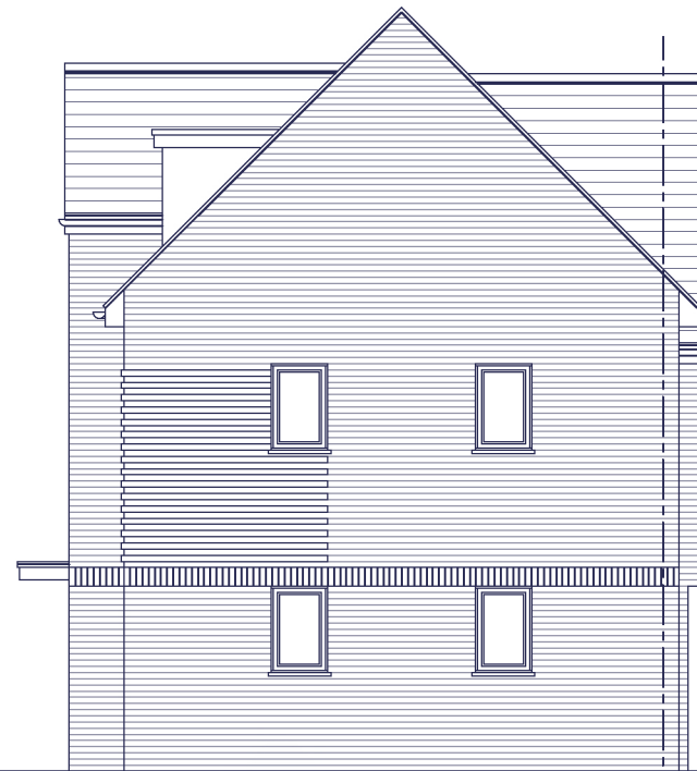
SIDE ELEVATION
