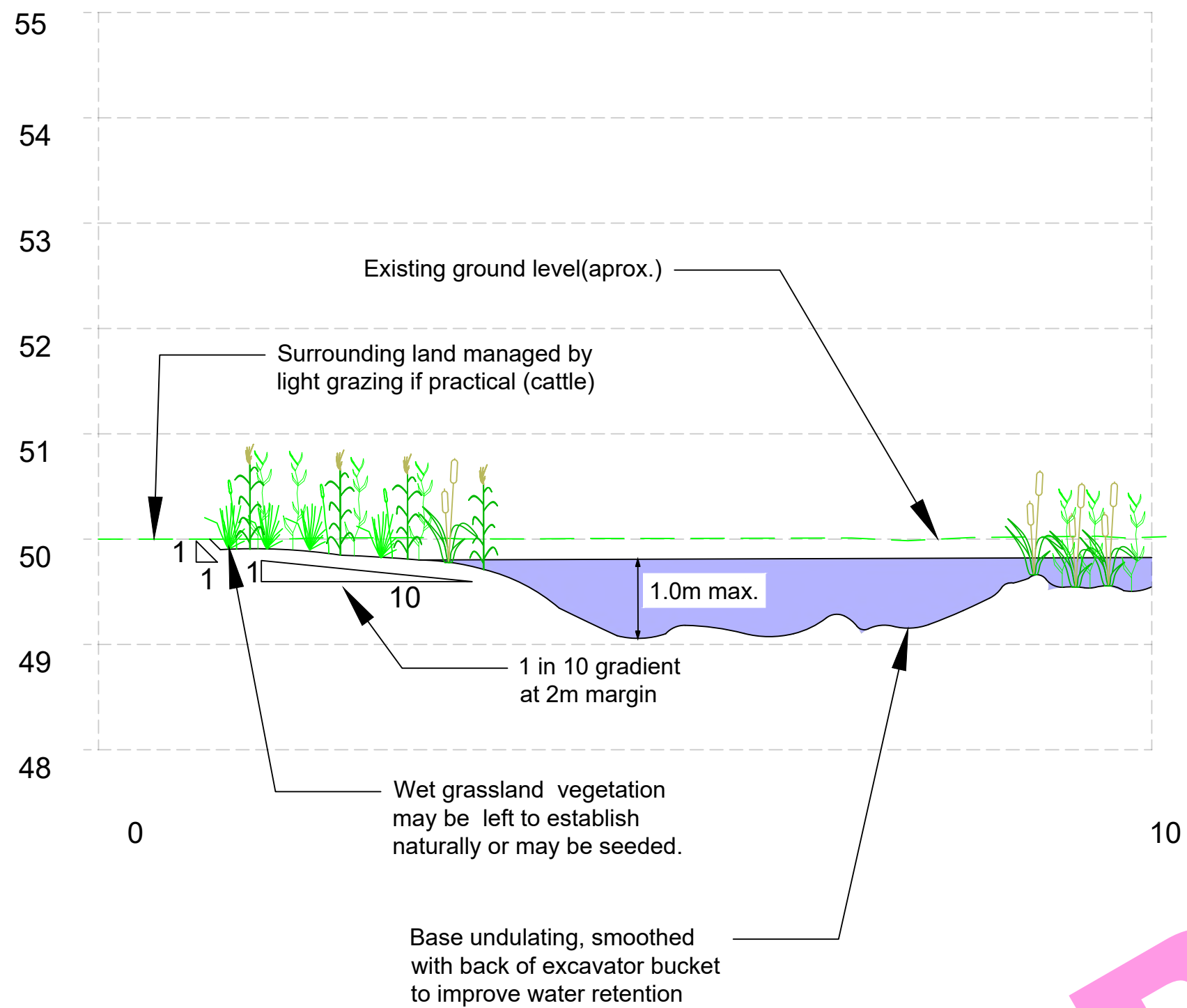
Typical section through flood plain scrape
