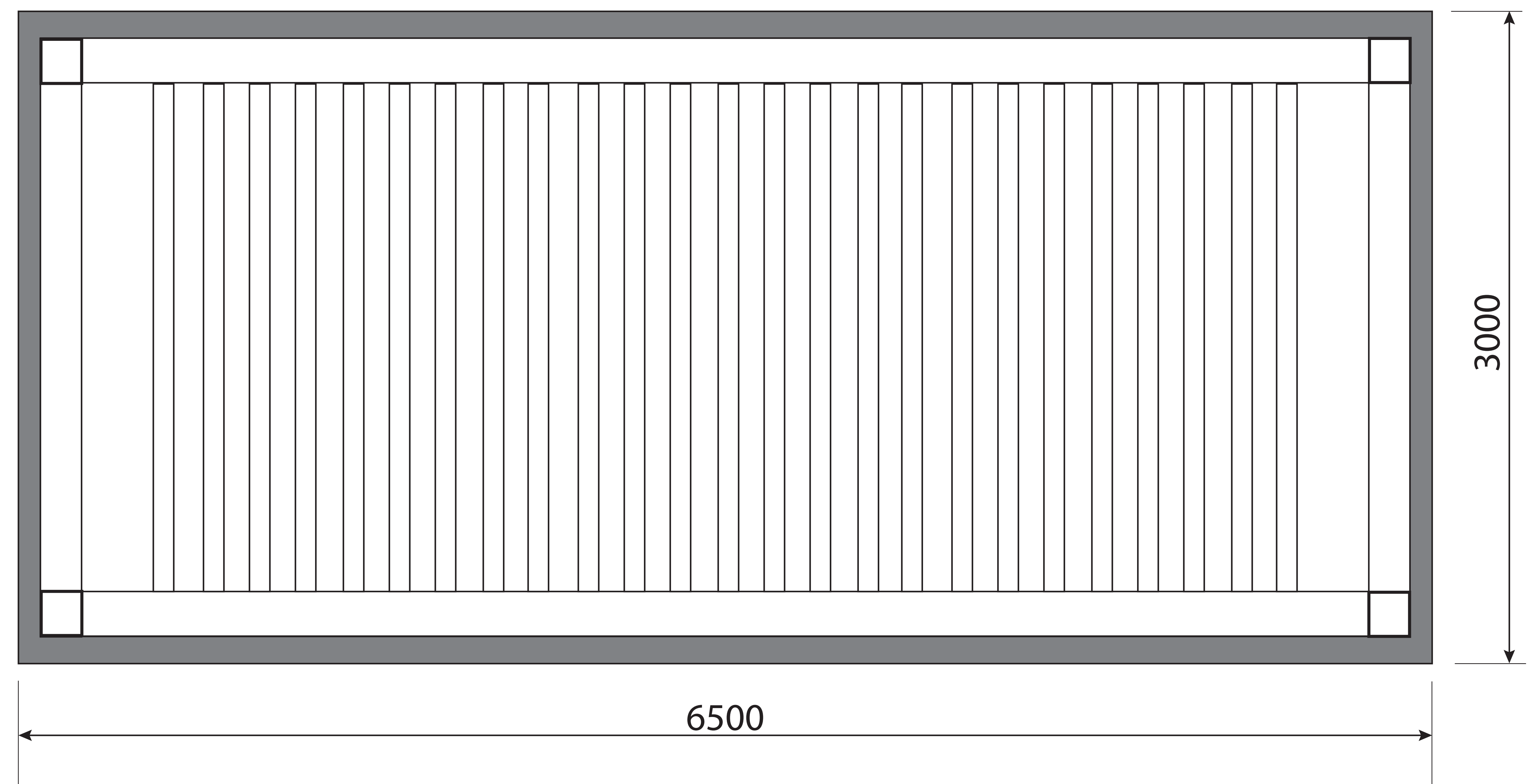
Refreshment Hut Slab Elevations & Cross Section
