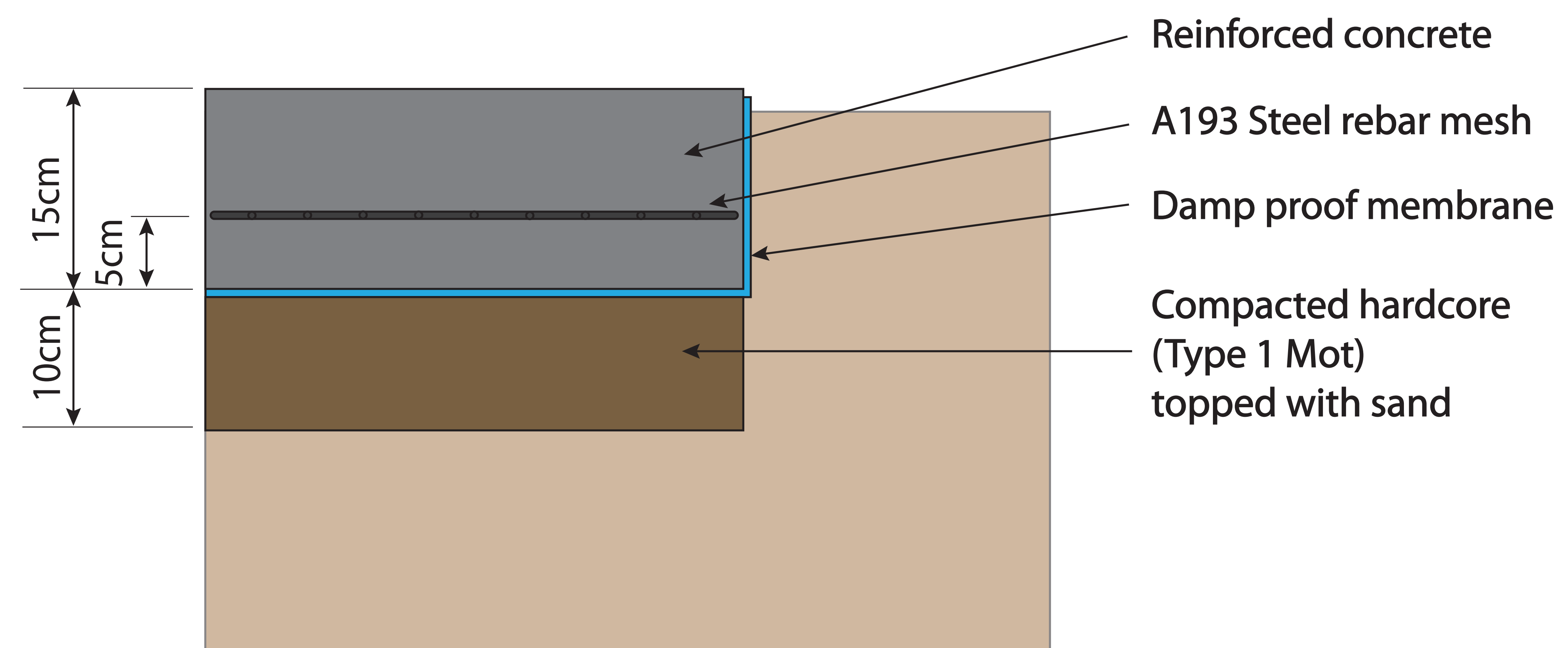
Base Slab Cross-section
