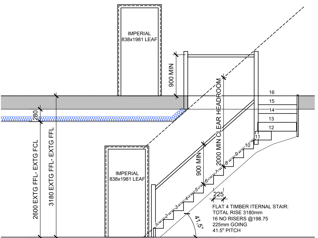
FLAT 3 STAIR COORDINATION SECTIONS
