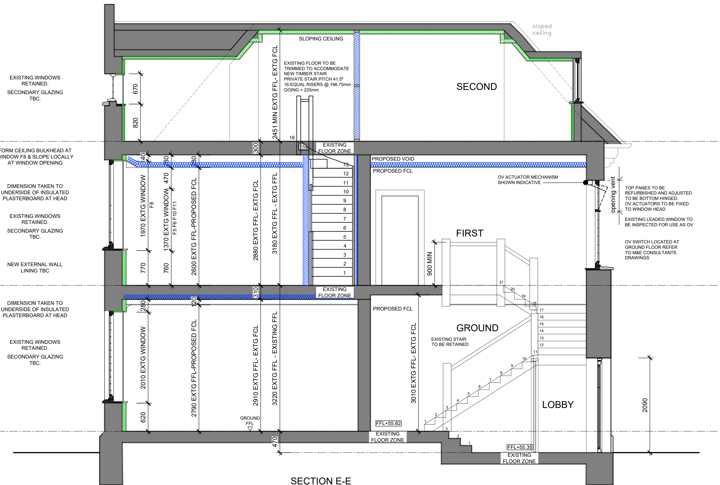
SECTION E-E
