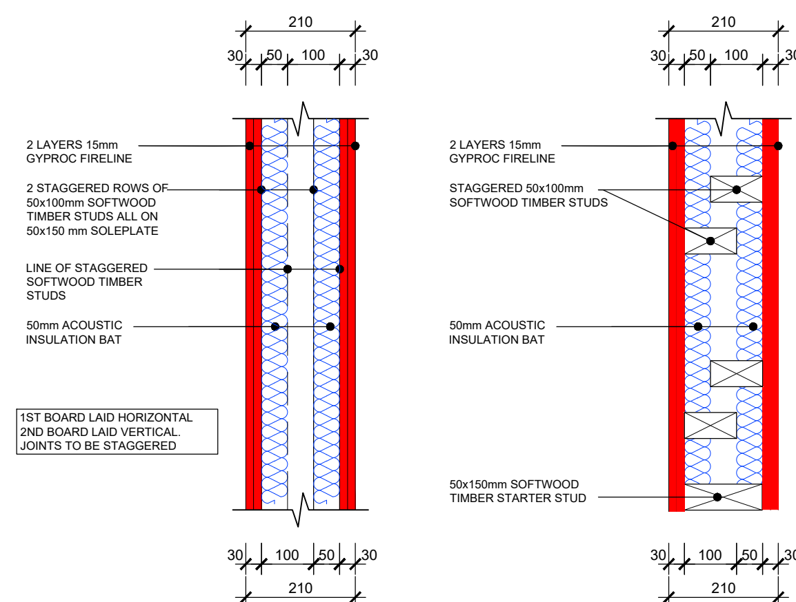
SEPARATING WALL SECTION
