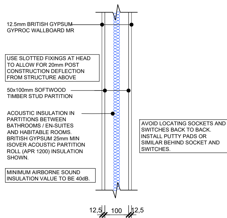
INTERNAL WALL
