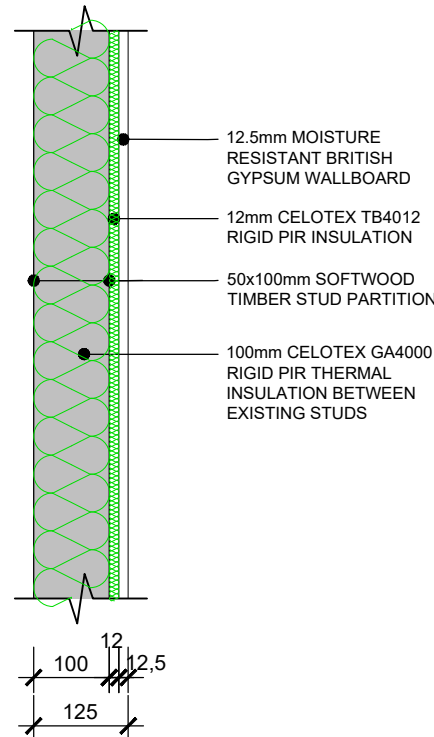
SECOND FLOOR ATTIC PARTITION AT BATHROOM
