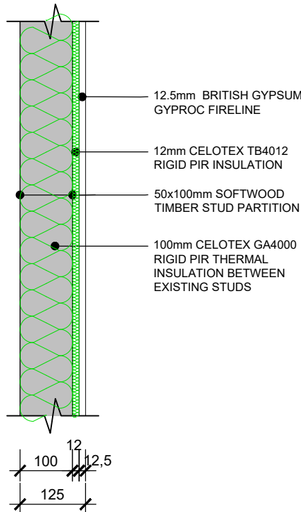
SECOND FLOOR ATTIC PARTITION AT STAIR LANDING
