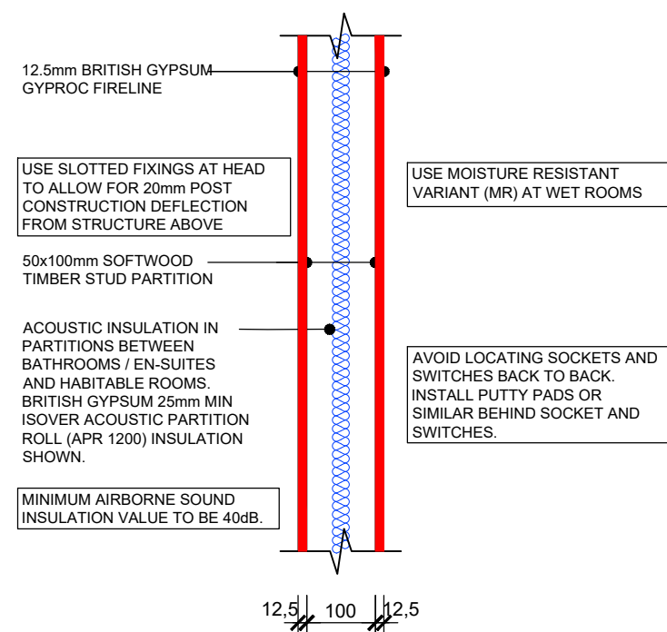
INTERNAL WALL
