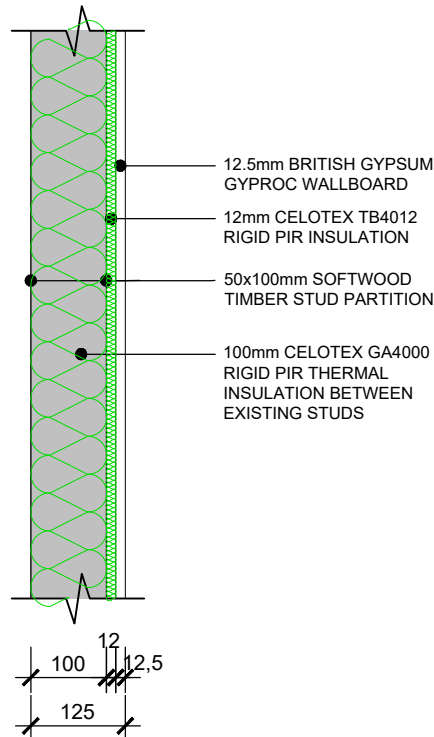
SECOND FLOOR ATTIC PARTITION
