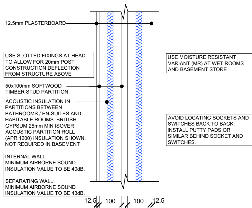
INFILL WALL
