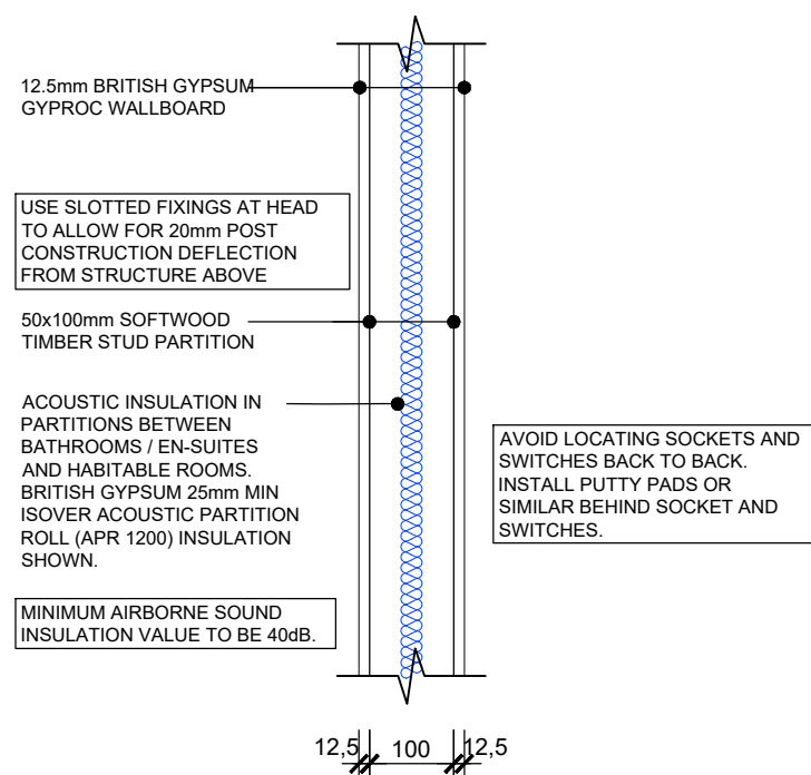
INTERNAL WALL
