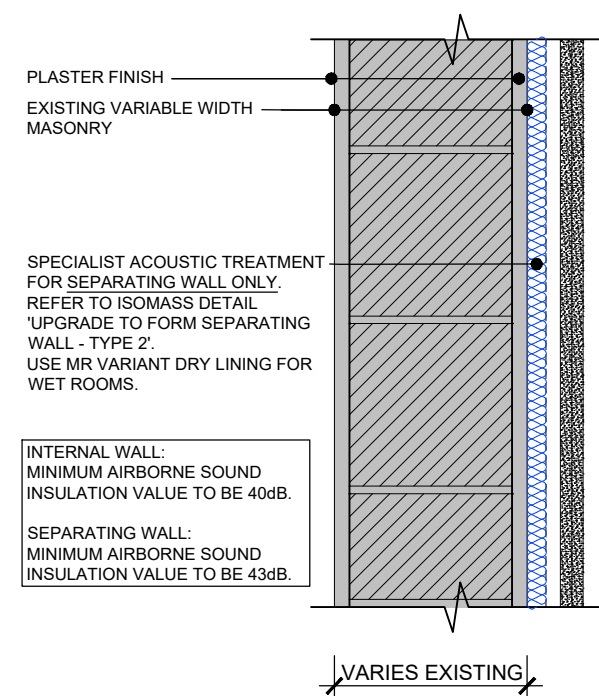
INTERNAL WALL & SEPARATING WALL
