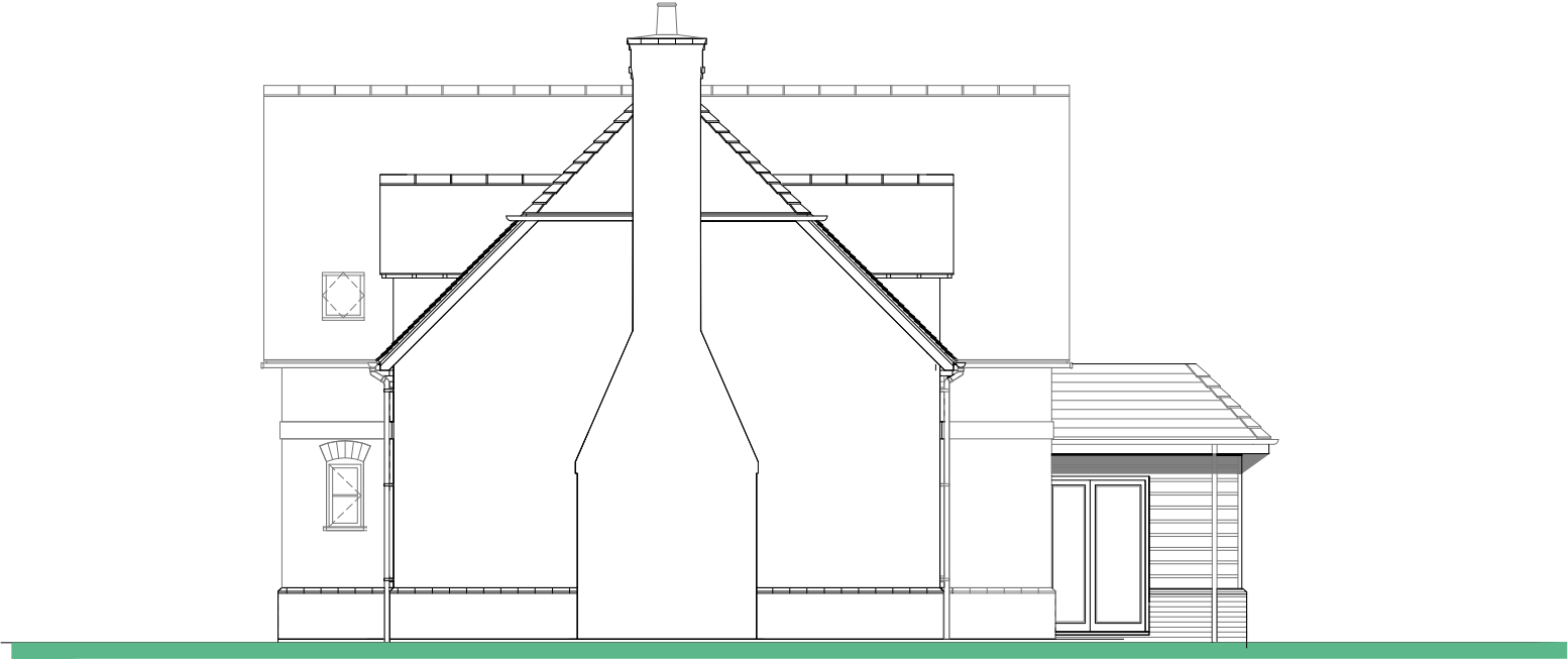
Side Elevation
