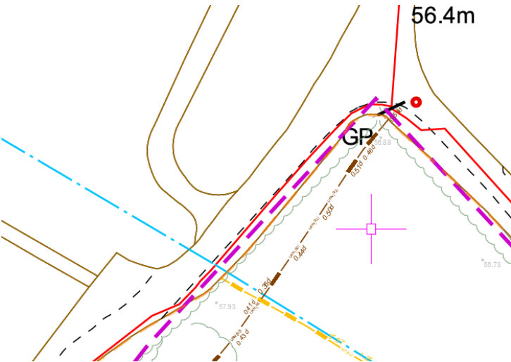
Figure 5 – SGN underground utility and survey area
