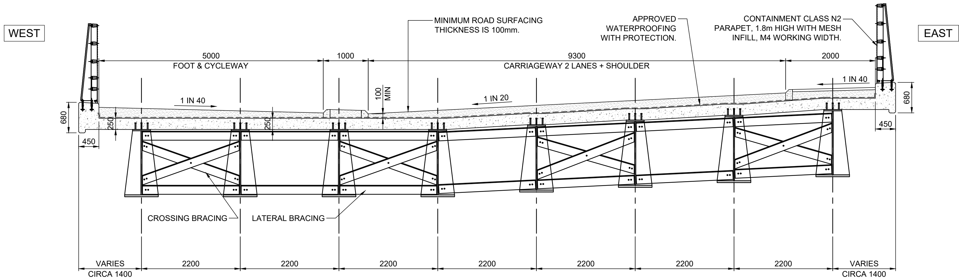
SECTION B-B (MID-SPAN) SCALE 1:50
