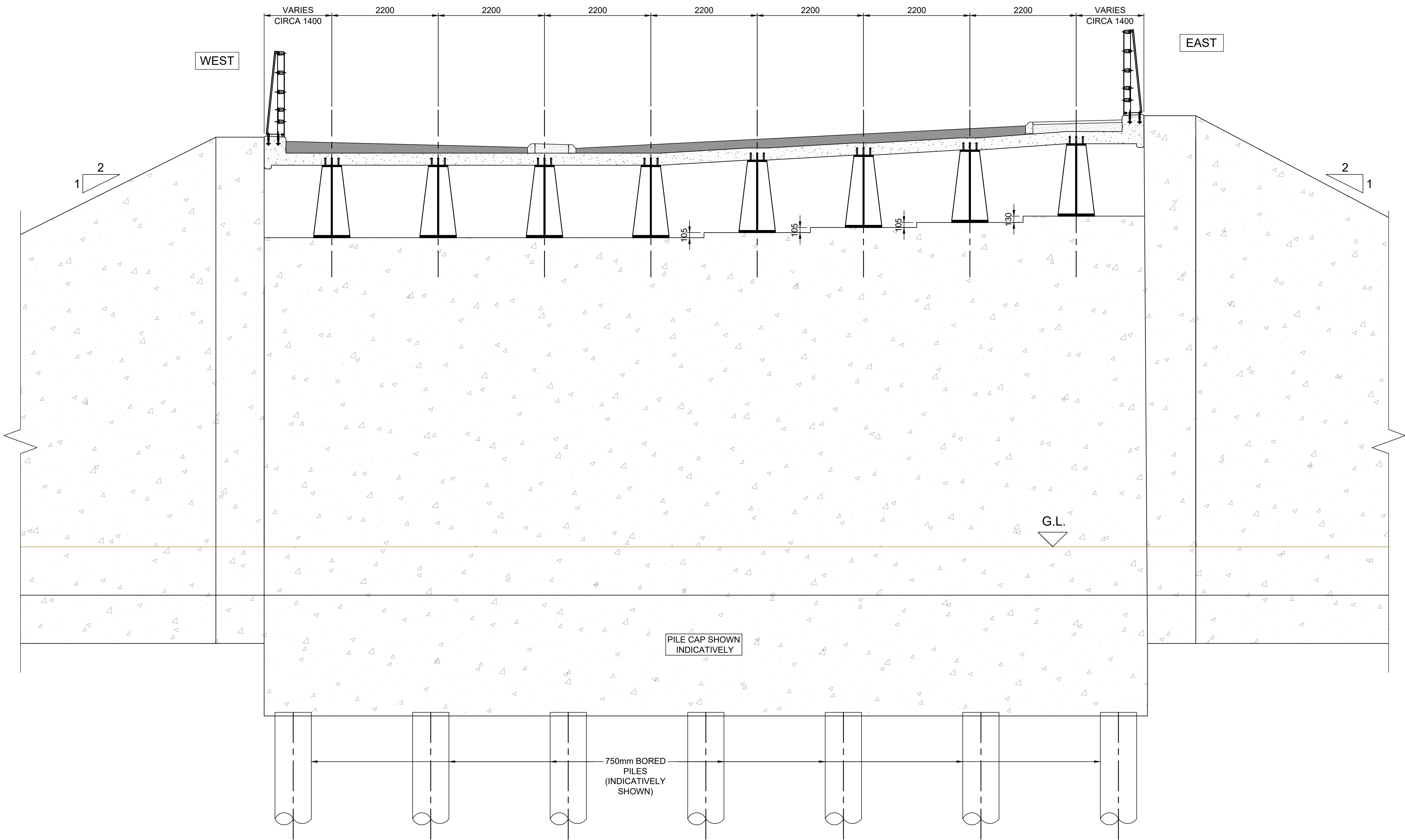
ELEVATION C-C (ABUTMENT) SCALE 1:50
