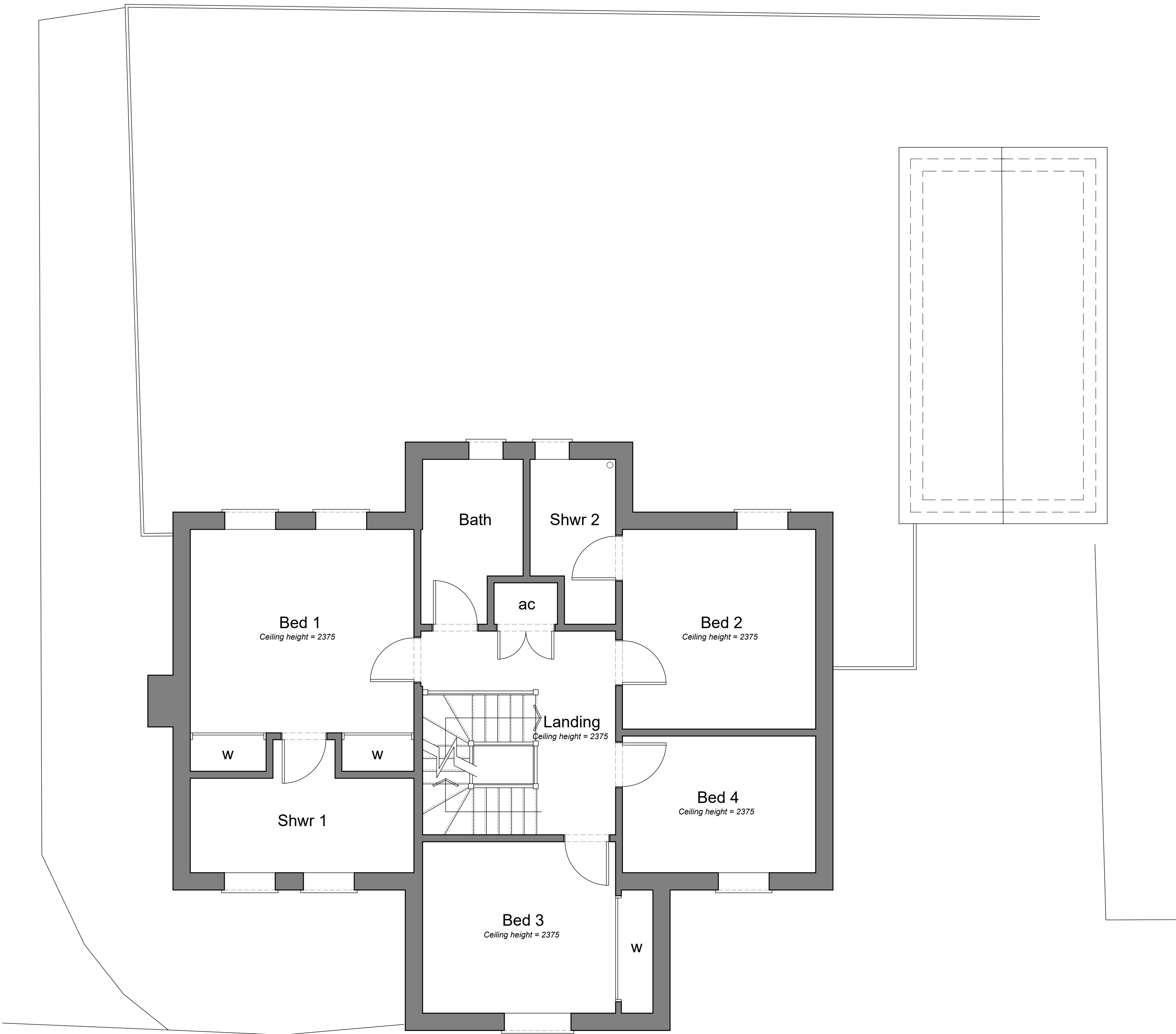
First Floor Plan 1:50 Scale
