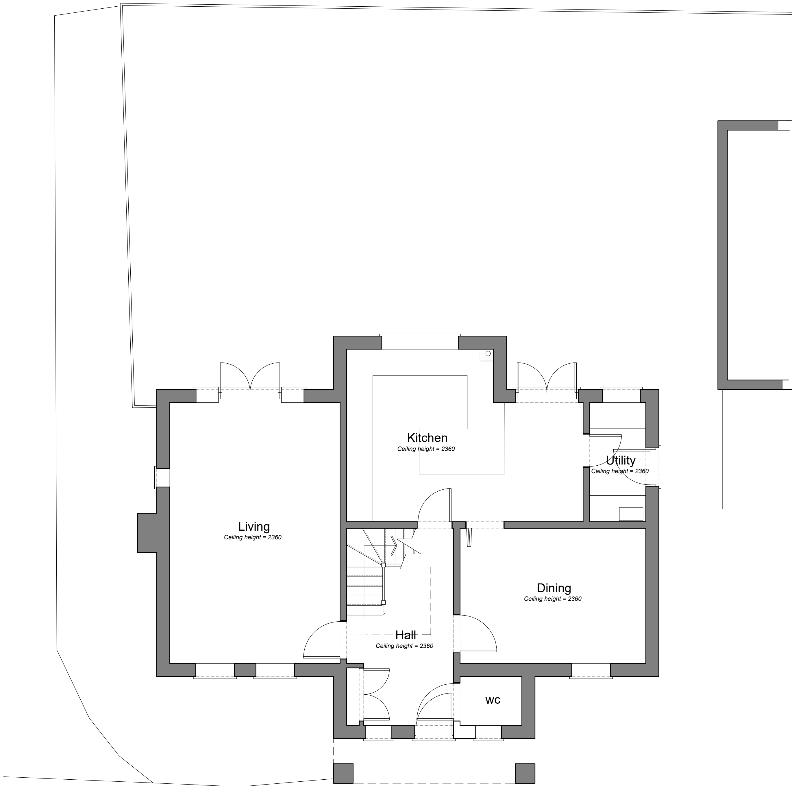
Ground Floor Plan 1:50 Scale
