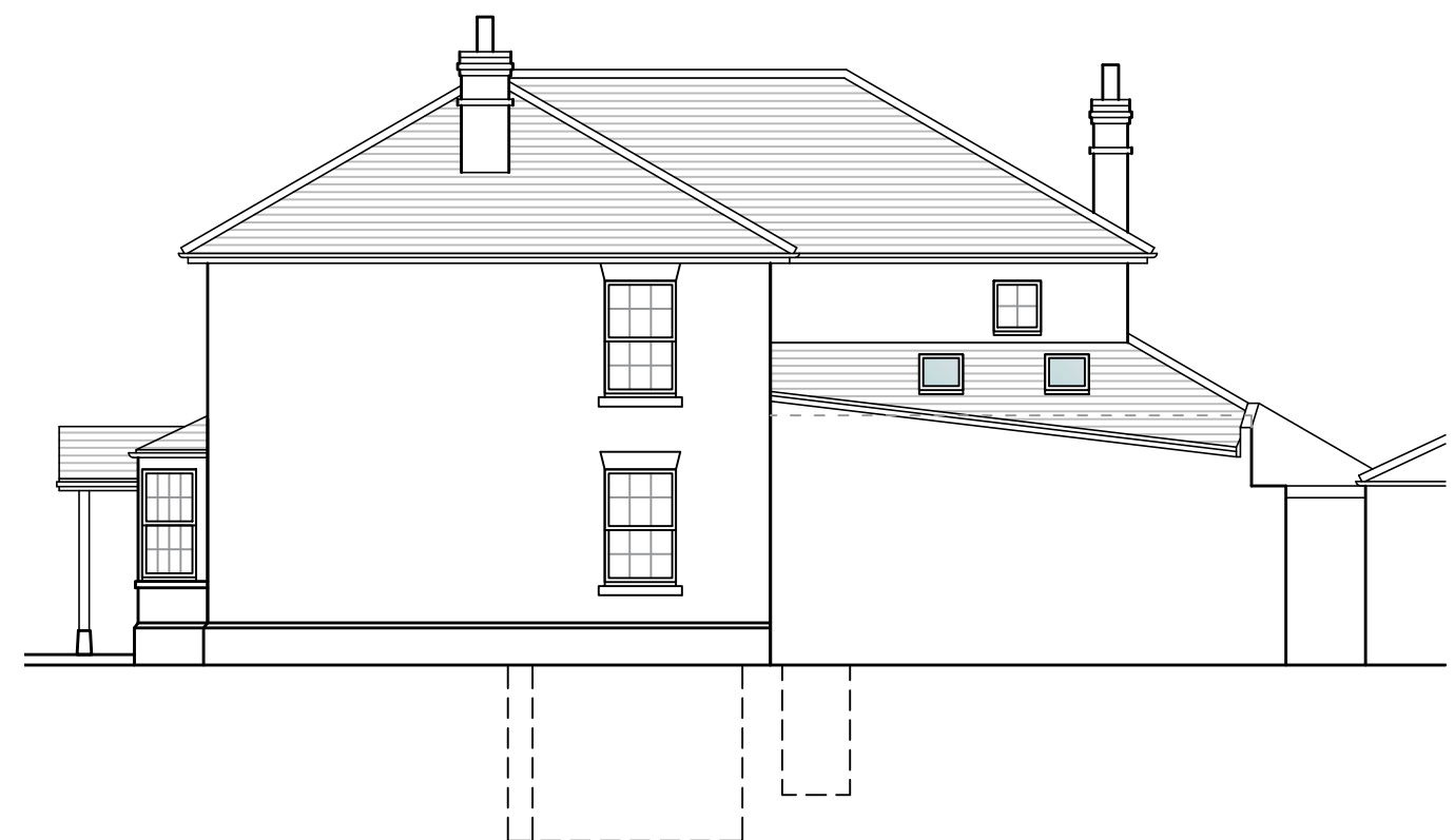
North Elevation
