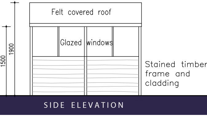
CAR & CYCLE PARKING STANDARD DOCUMENT. Design in accordance with section 4.7- CYCLE PARKING DESIGN
