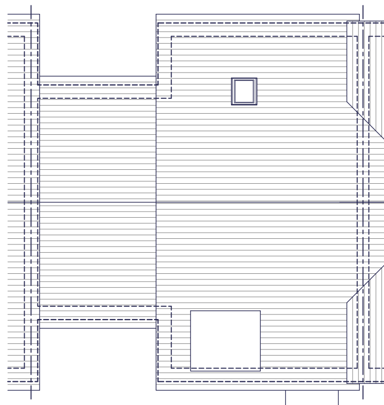
ROOF PLAN
