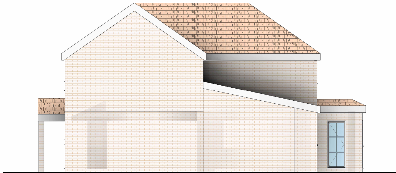
Existing Left View 1 : 100
