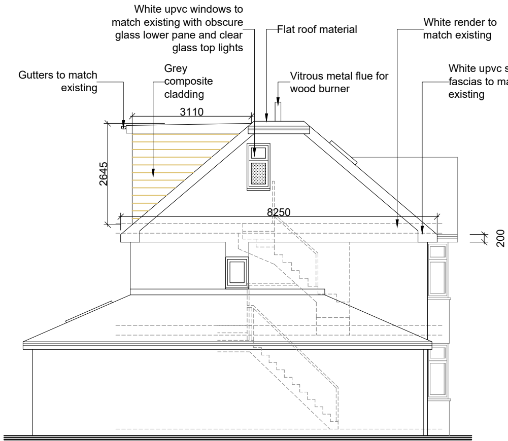
1:100 Proposed Lh side Elevation
