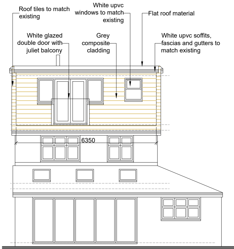
1:100 Proposed Rear Elevation
