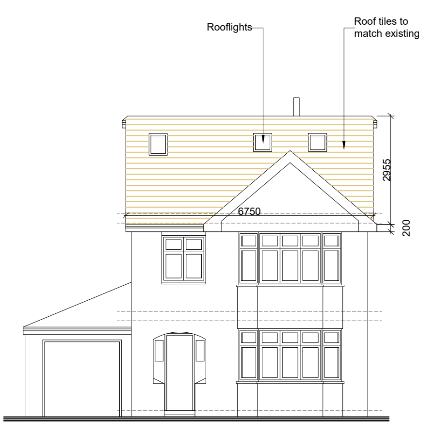
1:100 Proposed Front Elevation
