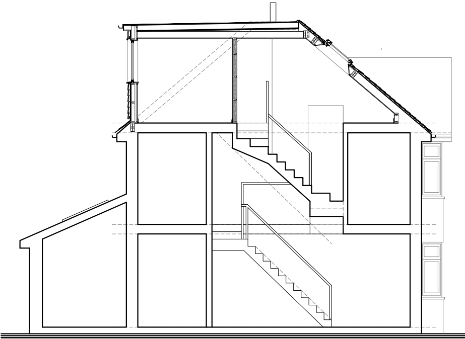
1:100 Proposed Side Section
