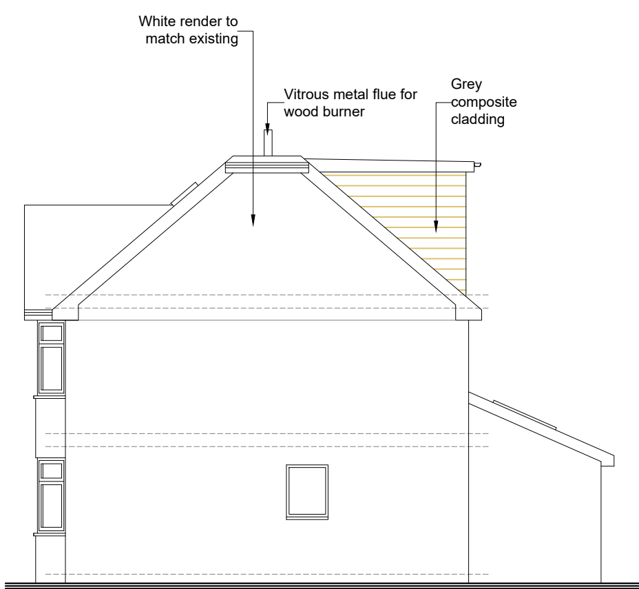
1:100 Proposed Rh side Elevation
