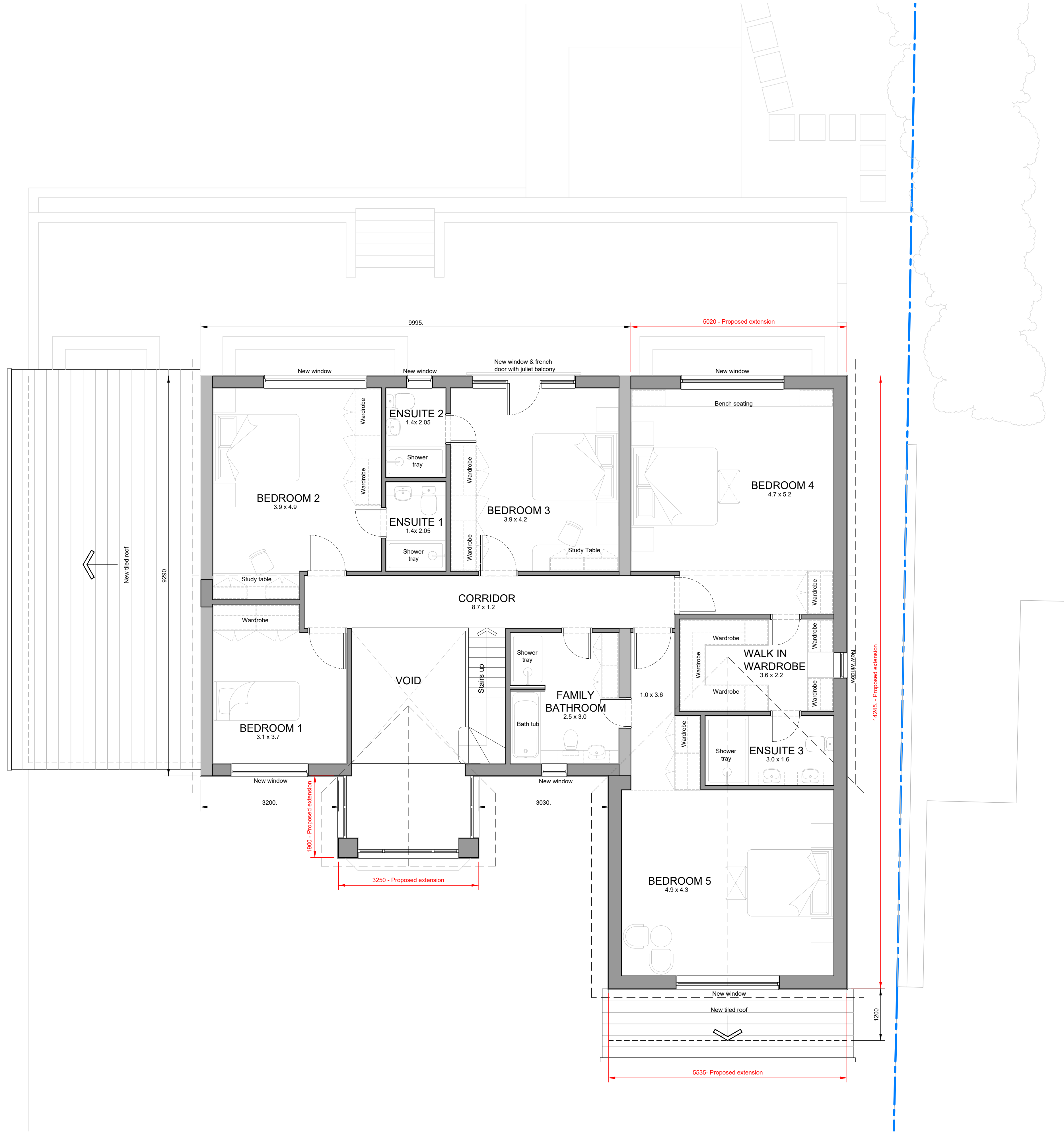
PROPOSED FIRST FLOOR PLAN
