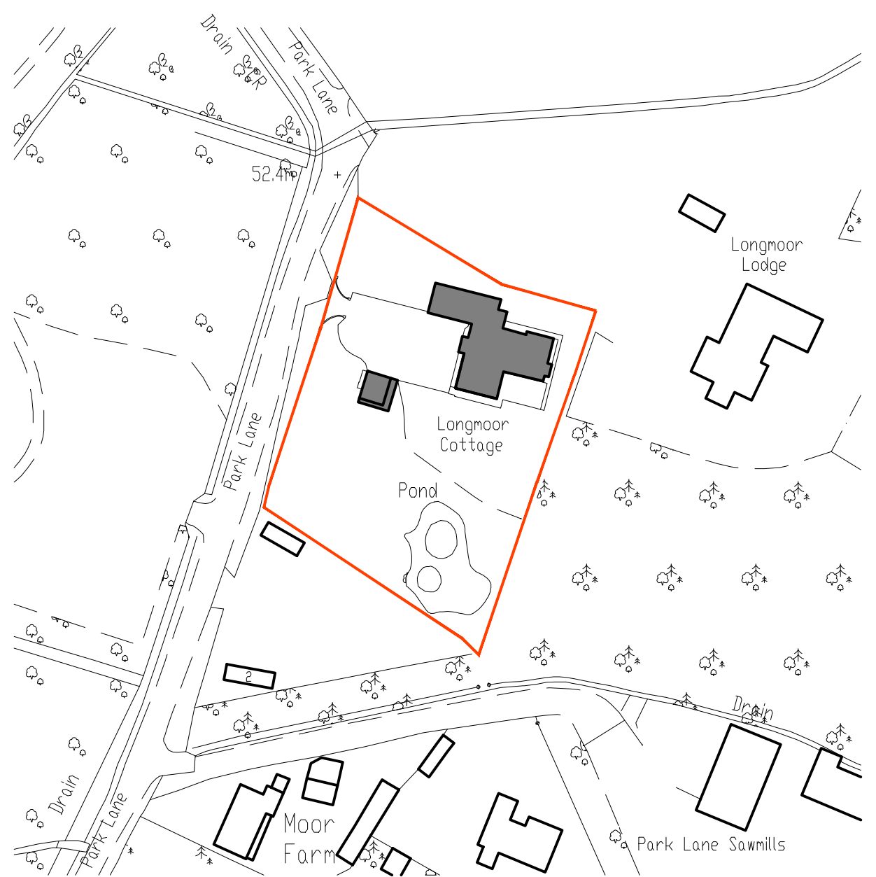
Location Plan 1:1250
