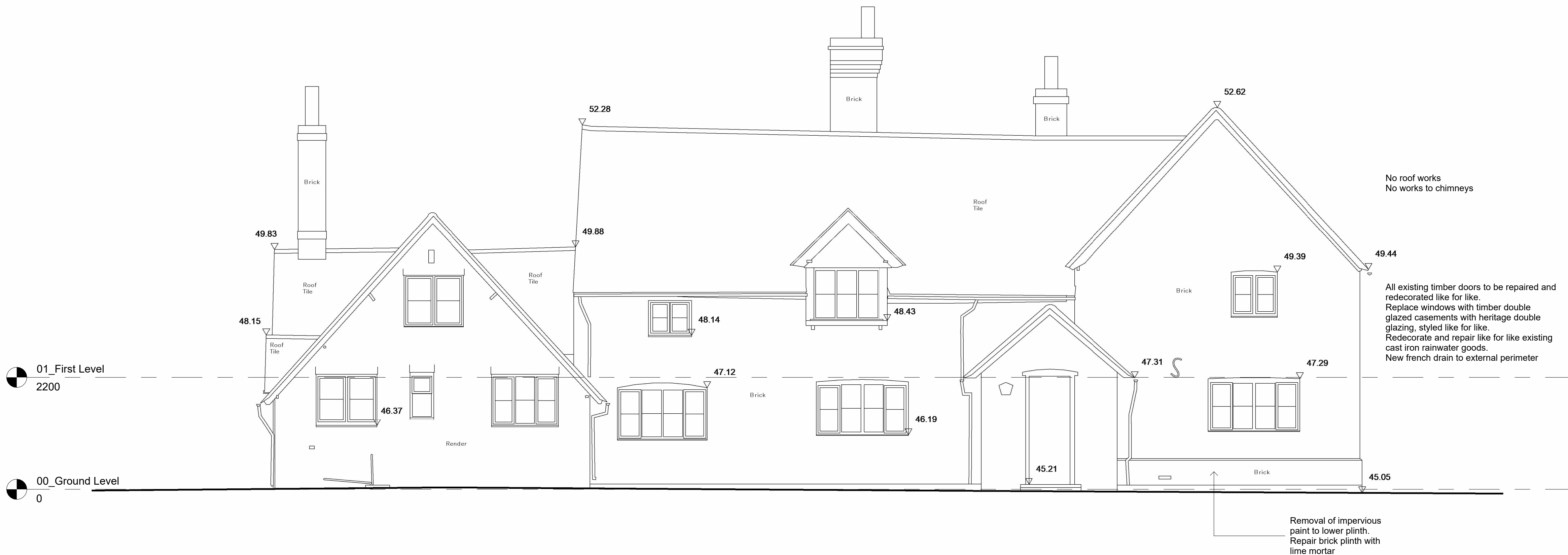
Proposed Farmhouse West Elevation 1 : 50
