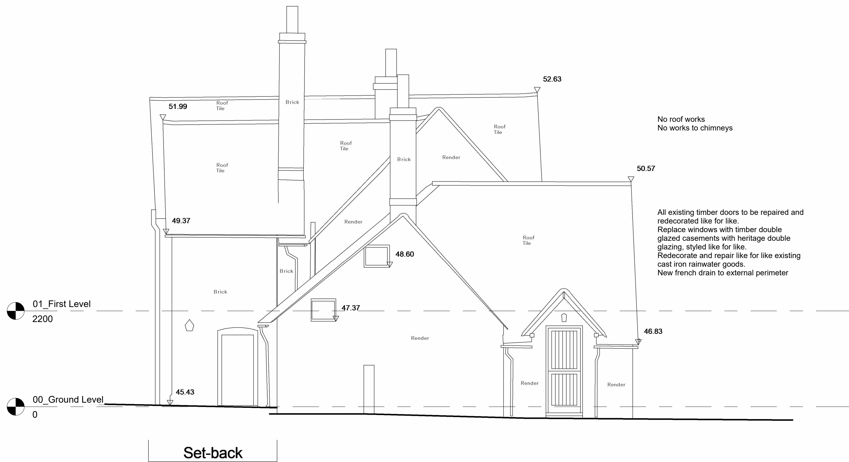
Proposed Farmhouse North Elevation 1 : 50
