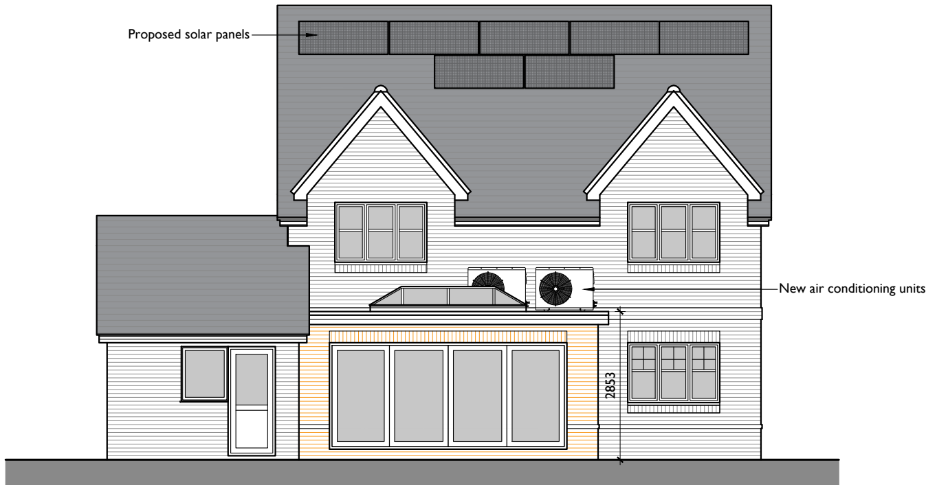
Rear Elevation: 1:100 at A3
