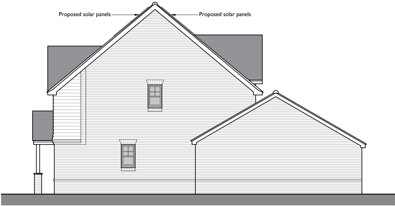
Side Elevation: RHS 1:100 at A3
